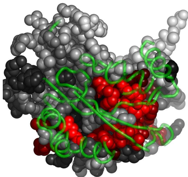
Fig. 5. Residues in 1u20A, at the interface with 1u20B, colored by their relative importance. 1u20B is shown in backbone representation (See Appendix for the coloring scheme for the protein chain 1u20A.)
