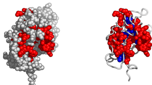
Fig. 7. A possible active surface on the chain 1u20A. The larger cluster it belongs to is shown in blue.
