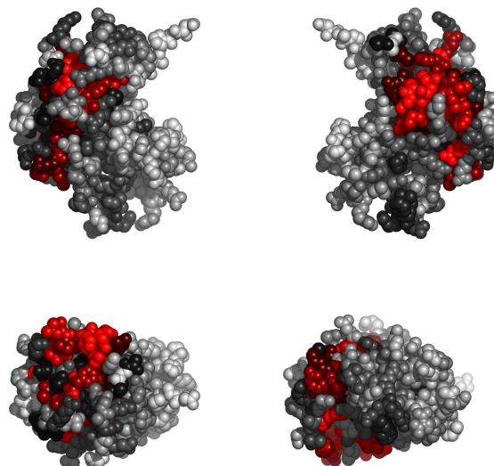
Fig. 1. Residues 14-209 in 1u20A colored by their relative importance. (See Appendix, Fig.8, for the coloring scheme.)
