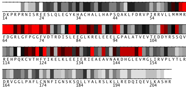
Fig. 1. Residues 14-209 in 1u20A colored by their relative importance. (See Appendix, Fig.8, for the coloring scheme.)
