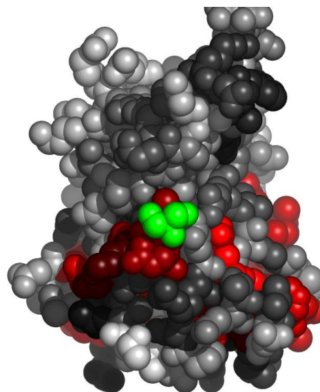
Fig. 6. Residues in 1u20A, at the interface with glycerol, colored by their relative importance. The ligand (glycerol) is colored green. Atoms further than 30 Å away from the geometric center of the ligand, as well as on the line of sight to the ligand were removed. (See Appendix for the coloring scheme for the protein chain 1u20A.)
