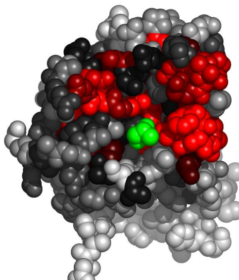
Fig. 4. Residues in 1u20A, at the interface with glycerol, colored by their relative importance. The ligand (glycerol) is colored green. Atoms further than 30Å away from the geometric center of the ligand, as well as on the line of sight to the ligand were removed. (See Appendix for the coloring scheme for the protein chain 1u20A.)
