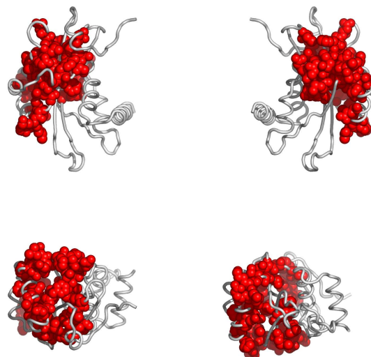
Fig. 2. Residues in 1u20A, colored by their relative importance. Clockwise: front, back, top and bottom views.
