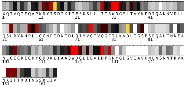
Fig. 1. Residues 1-165 in 1u4cB colored by their relative importance. (See Appendix, Fig.7, for the coloring scheme.)
