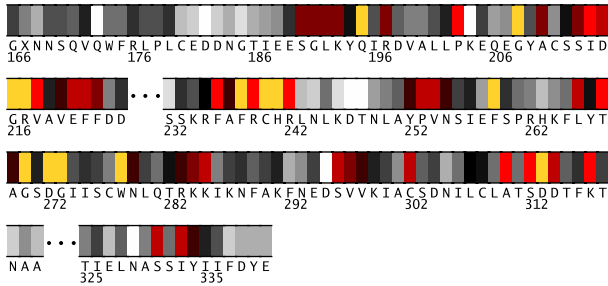
Fig. 2. Residues 166-340 in 1u4cB colored by their relative importance. (See Appendix, Fig.7, for the coloring scheme.)
