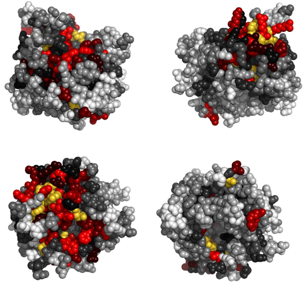
Fig. 3. Residues in 1u4cB, colored by their relative importance. Clockwise: front, back, top and bottom views.
