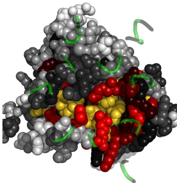
Fig. 5. Residues in 1u4cB, at the interface with 1u4cA, colored by their relative importance. 1u4cA is shown in backbone representation (See Appendix for the coloring scheme for the protein chain 1u4cB.)
