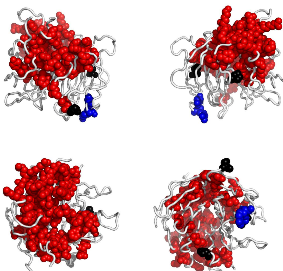
Fig. 4. Residues in 1u4cB, colored according to the cluster they belong to: red, followed by blue and yellow are the largest clusters (see Appendix for the coloring scheme). Clockwise: front, back, top and bottom views. The corresponding Pymol script is attached.
