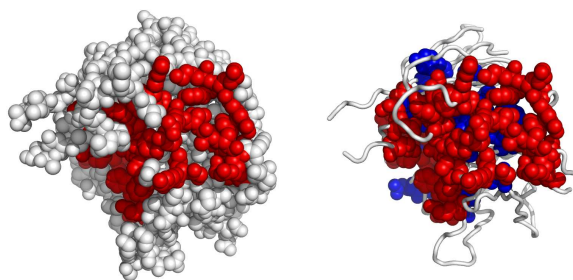
Fig. 6. A possible active surface on the chain 1u4cB. The larger cluster it belongs to is shown in blue.
