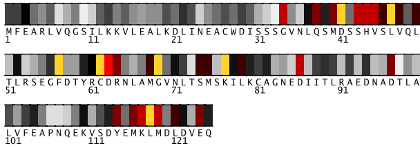
Fig. 1. Residues 1-125 in 1u7bA colored by their relative importance. (See Appendix, Fig.11, for the coloring scheme.)
