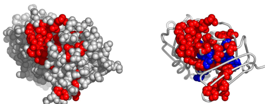
Fig. 10. Another possible active surface on the chain 1u7bA. The larger cluster it belongs to is shown in blue.
