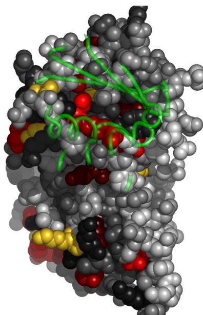
Fig. 7. Residues in 1u7bA, at the interface with 1u7bA2, colored by their relative importance. 1u7bA2 is shown in backbone representation (See Appendix for the coloring scheme for the protein chain 1u7bA.)
