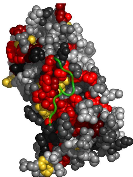
Fig. 5. Residues in 1u7bA, at the interface with 1u7bB, colored by their relative importance. 1u7bB is shown in backbone representation (See Appendix for the coloring scheme for the protein chain 1u7bA.)
