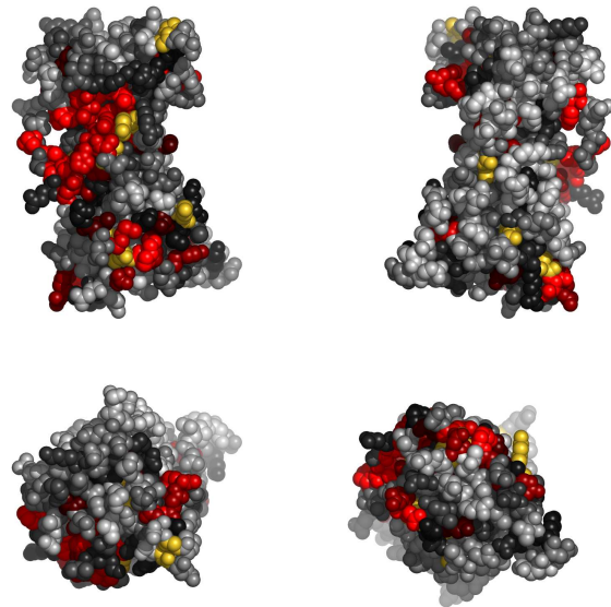
Fig. 3. Residues in 1u7bA, colored by their relative importance. Clockwise: front, back, top and bottom views.
