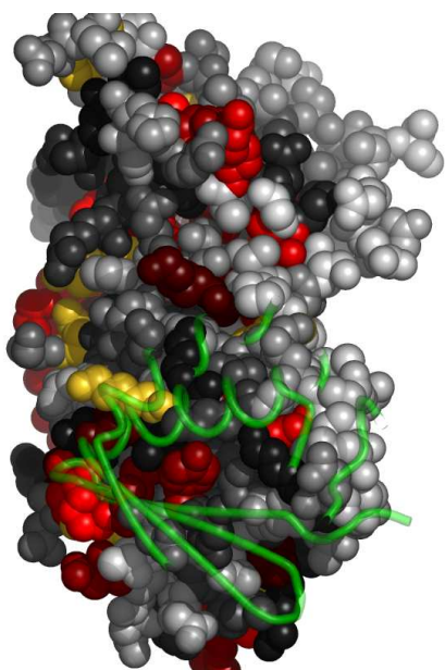
Fig. 6. Residues in 1u7bA, at the interface with 1u7bA1, colored by their relative importance. 1u7bA1 is shown in backbone representation (See Appendix for the coloring scheme for the protein chain 1u7bA.)
