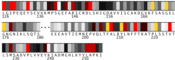
Fig. 2. Residues 126-255 in 1u7bA colored by their relative importance. (See Appendix, Fig.11, for the coloring scheme.)
