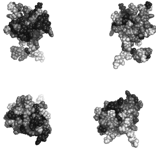
Fig. 2. Residues in luezA, colored by their relative importance. Clockwise: front, back, top and bottom views.
