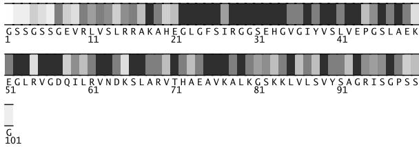
Fig. 1. Residues 1-101 in luezA colored by their relative importance. (See Appendix, Fig.4, for the coloring scheme.)
