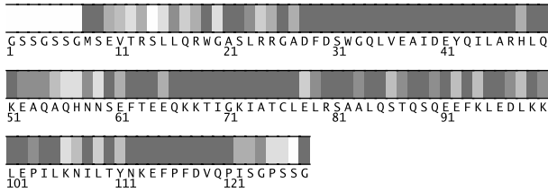
Fig. 1. Residues 1-128 in Iug7A colored by their relative importance. (See Appendix, Fig.4, for the coloring scheme.)
