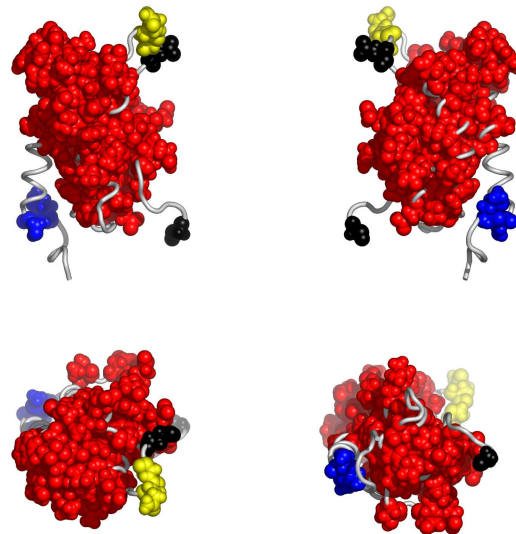
Fig. 2. Residues in Iug7A, colored by their relative importance. Clockwise: front, back, top and bottom views.
