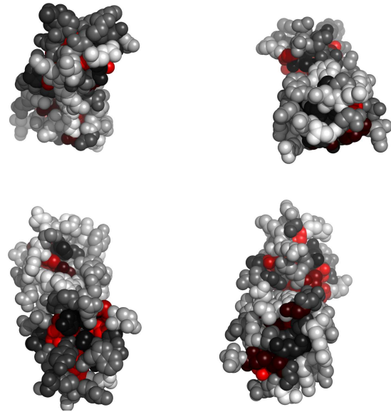
Fig. 2. Residues in 1uuaA, colored by their relative importance. Clockwise: front, back, top and bottom views.
