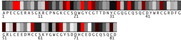
Fig. 1. Residues 1-82 in 1uuaA colored by their relative importance. (See Appendix, Fig.5, for the coloring scheme.)
