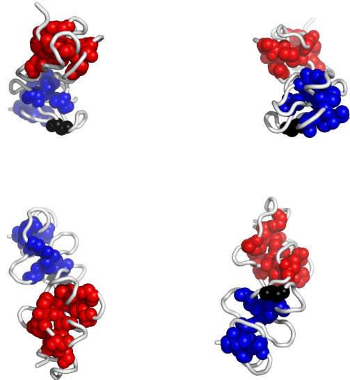
Fig. 3. Residues in 1uuaA, colored according to the cluster they belong to: red, followed by blue and yellow are the largest clusters (see Appendix for the coloring scheme). Clockwise: front, back, top and bottom views. The corresponding Pymol script is attached.
