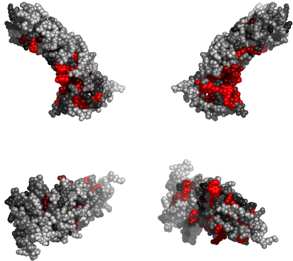
Fig. 3. Residues in lupkA, colored by their relative importance. Clockwise: front, back, top and bottom views.
