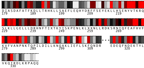
Fig. 2. Residues 179-339 in lupkA colored by their relative importance. (See Appendix, Fig.8, for the coloring scheme.)
