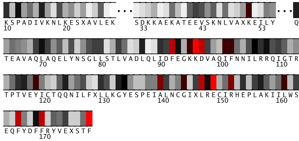
Fig. 1. Residues 10-178 in lupkA colored by their relative importance. (See Appendix, Fig.8, for the coloring scheme.)
