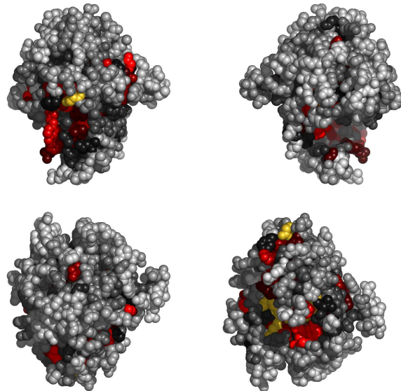
Fig. 3. Residues in 1v19A, colored by their relative importance. Clockwise: front, back, top and bottom views.
