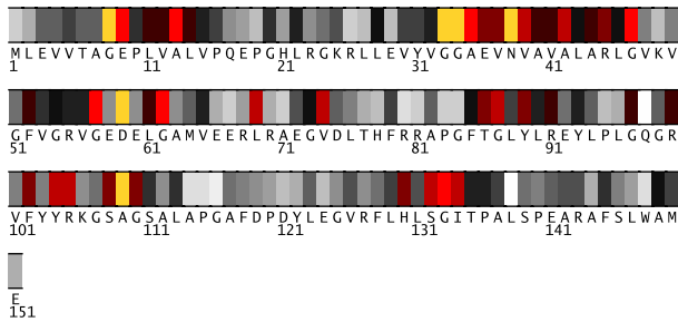
Fig. 1. Residues 1-151 in 1v19A colored by their relative importance. (See Appendix, Fig.11, for the coloring scheme.)
