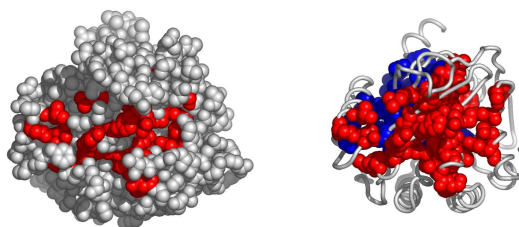
Fig. 10. Another possible active surface on the chain 1v19A. The larger cluster it belongs to is shown in blue.
