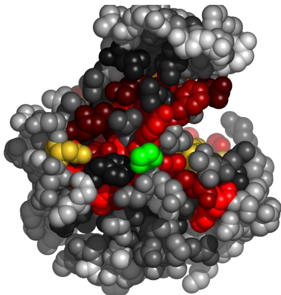
Fig. 8. Residues in 1v19A, at the interface with DIO, colored by their relative importance. The ligand (DIO) is colored green. Atoms further than 30Å away from the geometric center of the ligand, as well as on the line of sight to the ligand were removed. (See Appendix for the coloring scheme for the protein chain 1v19A.)
