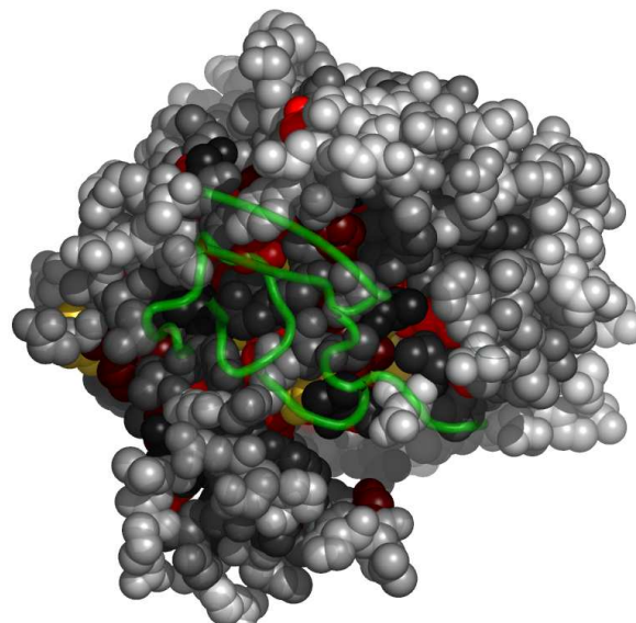
Fig. 7. Residues in 1v19A, at the interface with 1v19A2, colored by their relative importance. 1v19A2 is shown in backbone representation (See Appendix for the coloring scheme for the protein chain 1v19A.)
