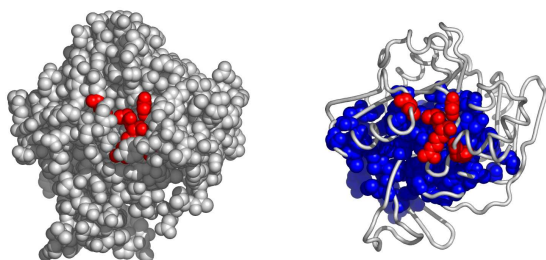
Fig. 9. A possible active surface on the chain 1v19A. The larger cluster it belongs to is shown in blue.
