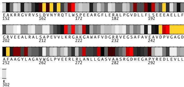
Fig. 2. Residues 152-302 in 1v19A colored by their relative importance. (See Appendix, Fig.11, for the coloring scheme.)
