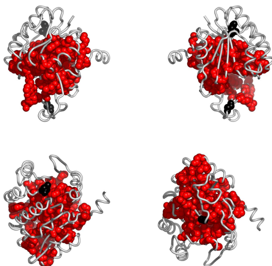
Fig. 4. Residues in 1v19A, colored according to the cluster they belong to: red, followed by blue and yellow are the largest clusters (see Appendix for the coloring scheme). Clockwise: front, back, top and bottom views. The corresponding Pymol script is attached.
