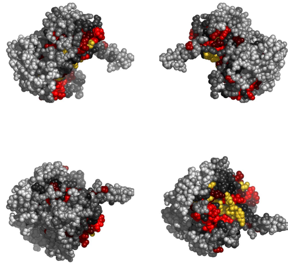
Fig. 3. Residues in 1v53A, colored by their relative importance. Clockwise: front, back, top and bottom views.
