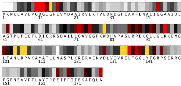
Fig. 1. Residues 1-178 in 1v53A colored by their relative importance. (See Appendix, Fig.7, for the coloring scheme.)
