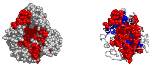
Fig. 6. A possible active surface on the chain 1v53A. The larger cluster it belongs to is shown in blue.
