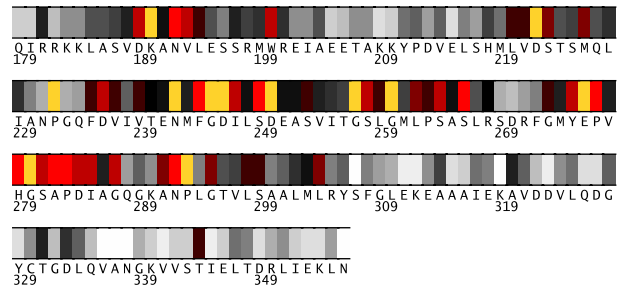
Fig. 2. Residues 179-356 in 1v53A colored by their relative importance. (See Appendix, Fig.7, for the coloring scheme.)
