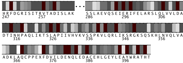
Fig. 2. Residues 247-403 in 1vyvB colored by their relative importance. (See Appendix, Fig.9, for the coloring scheme.)
