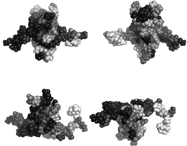
Fig. 1. Residues 1-76 in 1vzsA colored by their relative importance. (See Appendix, Fig.4, for the coloring scheme.)
