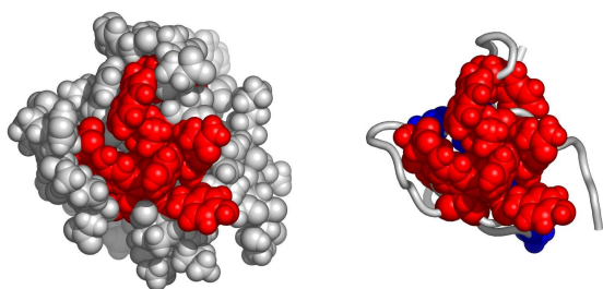
Fig. 4. A possible active surface on the chain 1w1fA. The larger cluster it belongs to is shown in blue.
