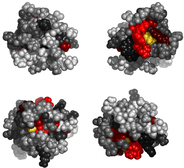
Fig. 2. Residues in 1w1fA, colored by their relative importance. Clockwise: front, back, top and bottom views.
