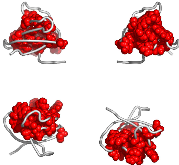
Fig. 3. Residues in 1w1fA, colored according to the cluster they belong to: red, followed by blue and yellow are the largest clusters (see Appendix for the coloring scheme). Clockwise: front, back, top and bottom views. The corresponding Pymol script is attached.
