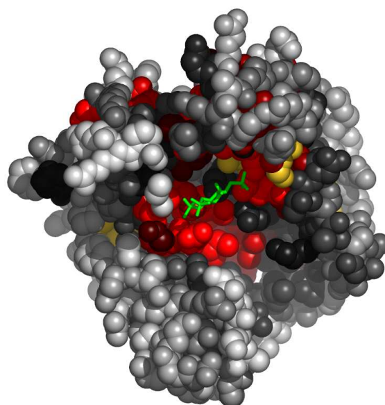
Fig. 6. Residues in 1w2cA, at the interface with I3P, colored by their relative importance. The ligand (I3P) is colored green. Atoms further than 30Å away from the geometric center of the ligand, as well as on the line of sight to the ligand were removed. (See Appendix for the coloring scheme for the protein chain 1w2cA.)
