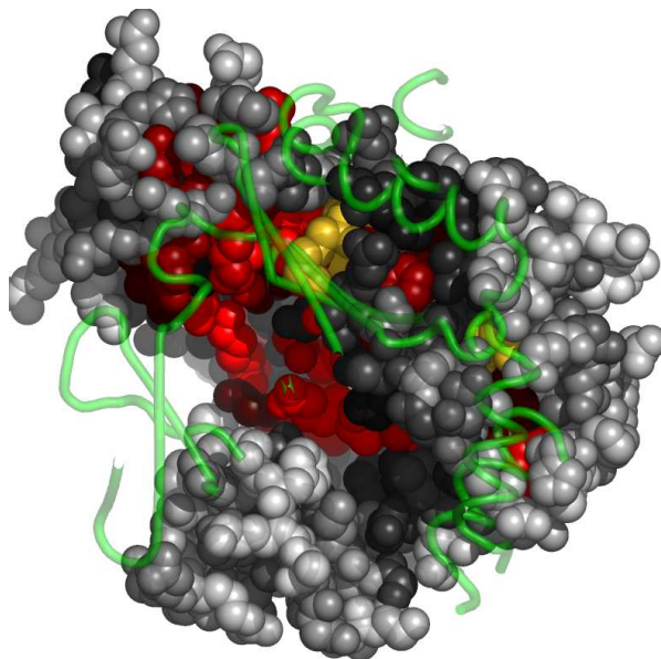
Fig. 5. Residues in 1w2cA, at the interface with 1w2cB, colored by their relative importance. 1w2cB is shown in backbone representation (See Appendix for the coloring scheme for the protein chain 1w2cA.)
