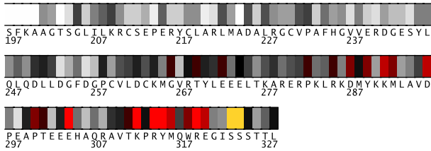
Fig. 1. Residues 197-328 in 1w2cA colored by their relative importance. (See Appendix, Fig.10, for the coloring scheme.)
