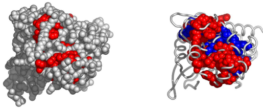
Fig. 9. A possible active surface on the chain 1w2cA. The larger cluster it belongs to is shown in blue.
