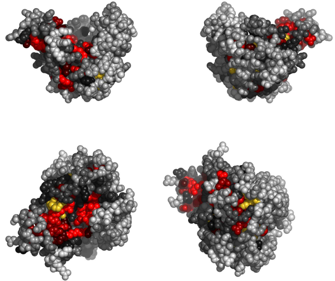
Fig. 3. Residues in 1w2cA, colored by their relative importance. Clockwise: front, back, top and bottom views.
