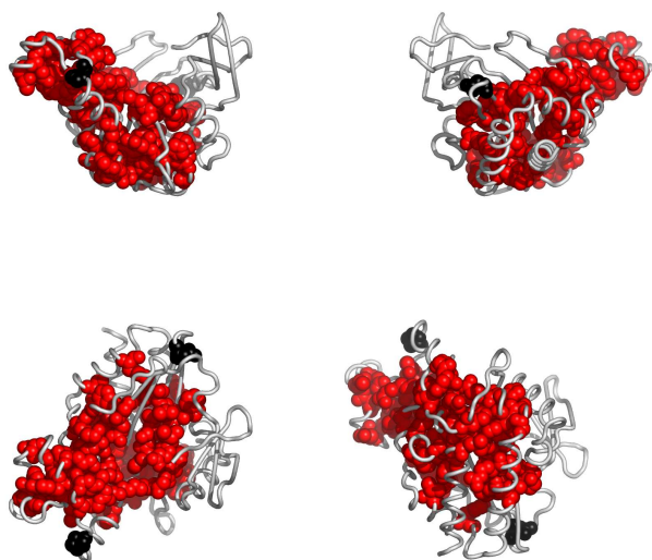
Fig. 4. Residues in 1w2cA, colored according to the cluster they belong to: red, followed by blue and yellow are the largest clusters (see Appendix for the coloring scheme). Clockwise: front, back, top and bottom views. The corresponding Pymol script is attached.
