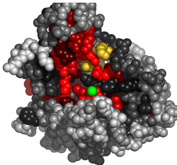
Fig. 7. Residues in 1w2cA, at the interface with ANP, colored by their relative importance. The ligand (ANP) is colored green. Atoms further than 30Å away from the geometric center of the ligand, as well as on the line of sight to the ligand were removed. (See Appendix for the coloring scheme for the protein chain 1w2cA.)
