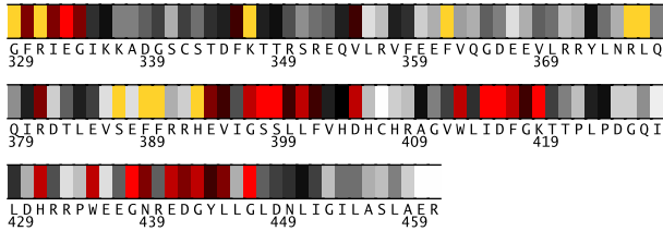
Fig. 2. Residues 329-461 in 1w2cA colored by their relative importance. (See Appendix, Fig.10, for the coloring scheme.)
