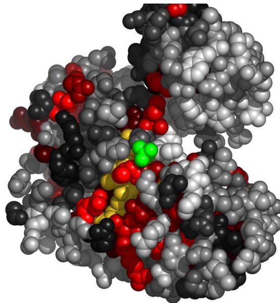
Fig. 6. Residues in 1w5sB, at the interface with sulfate ion, colored by their relative importance. The ligand (sulfate ion) is colored green. Atoms further than 30Å away from the geometric center of the ligand, as well as on the line of sight to the ligand were removed. (See Appendix for the coloring scheme for the protein chain 1w5sB.)
