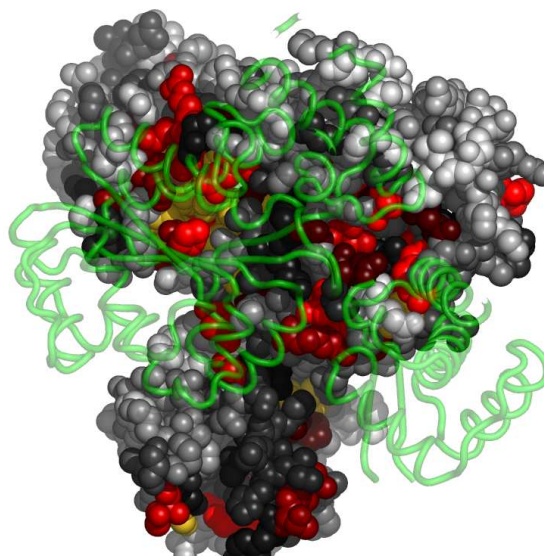
Fig. 7. Residues in 1w5sB, at the interface with 1w5sA, colored by their relative importance. 1w5sA is shown in backbone representation (See Appendix for the coloring scheme for the protein chain 1w5sB.)
