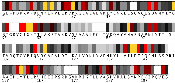
Fig. 1. Residues 7-204 in 1w5sB colored by their relative importance. (See Appendix, Fig.10, for the coloring scheme.)
