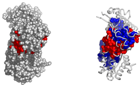
Fig. 8. A possible active surface on the chain 1w5sB. The larger cluster it belongs to is shown in blue.
