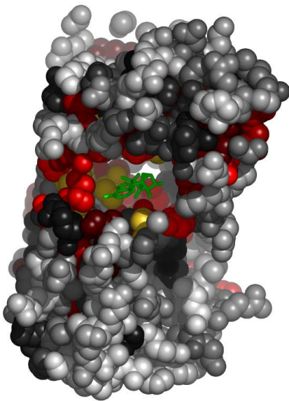
Fig. 5. Residues in 1w5sB, at the interface with ADP, colored by their relative importance. The ligand (ADP) is colored green. Atoms further than 30Å away from the geometric center of the ligand, as well as on the line of sight to the ligand were removed. (See Appendix for the coloring scheme for the protein chain 1w5sB.)
