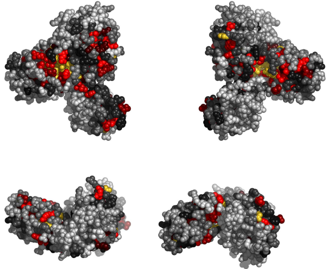
Fig. 1. Residues 7-204 in 1w5sB colored by their relative importance. (See Appendix, Fig.10, for the coloring scheme.)
