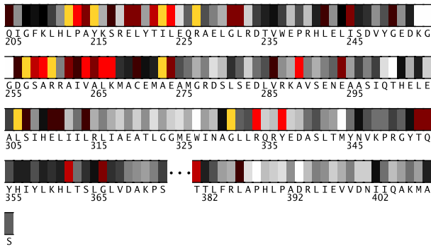
Fig. 2. Residues 205-409 in 1w5sB colored by their relative importance. (See Appendix, Fig.10, for the coloring scheme.)
