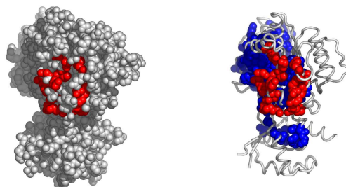
Fig. 9. Another possible active surface on the chain 1w5sB. The larger cluster it belongs to is shown in blue.
