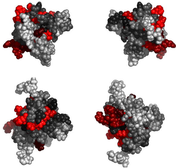
Fig. 2. Residues in 1wjnA, colored by their relative importance. Clockwise: front, back, top and bottom views.
