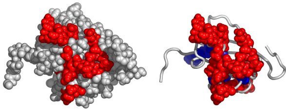
Fig. 4. A possible active surface on the chain 1wjnA. The larger cluster it belongs to is shown in blue.
