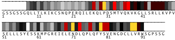
Fig. 1. Residues 1-97 in 1wjnA colored by their relative importance. (See Appendix, Fig.5, for the coloring scheme.)
