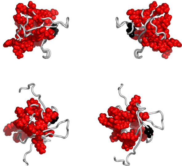
Fig. 3. Residues in 1wjnA, colored according to the cluster they belong to: red, followed by blue and yellow are the largest clusters (see Appendix for the coloring scheme). Clockwise: front, back, top and bottom views. The corresponding Pymol script is attached.
