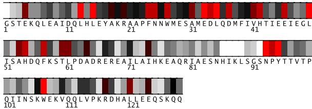
Fig. 1. Residues 1-129 in 1wlxA colored by their relative importance. (See Appendix, Fig.5, for the coloring scheme.)
