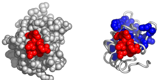
Fig. 6. A possible active surface on the chain 1wlzA. The larger cluster it belongs to is shown in blue.
