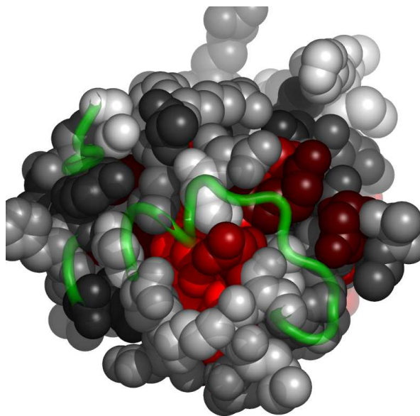
Fig. 5. Residues in 1wlzA, at the interface with 1wlzC, colored by their relative importance. 1wlzC is shown in backbone representation (See Appendix for the coloring scheme for the protein chain 1wlzA.)
