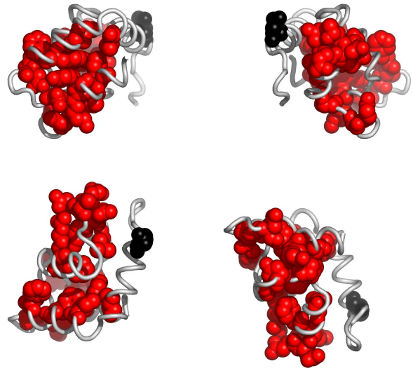
Fig. 3. Residues in 1wzA, colored according to the cluster they belong to: red, followed by blue and yellow are the largest clusters (see Appendix for the coloring scheme). Clockwise: front, back, top and bottom views. The corresponding Pymol script is attached.
