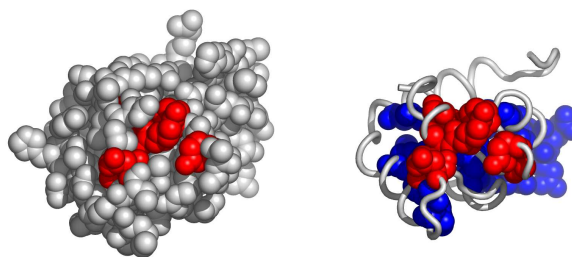
Fig. 7. Another possible active surface on the chain 1wlzA. The larger cluster it belongs to is shown in blue.
