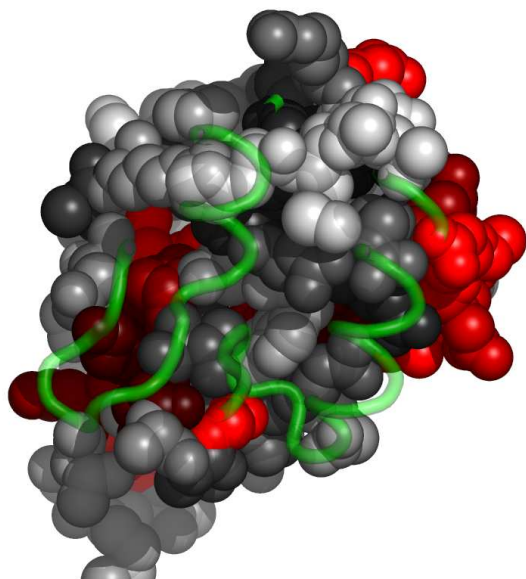
Fig. 4. Residues in 1wlzA, at the interface with 1wlzD, colored by their relative importance. 1wlzD is shown in backbone representation (See Appendix for the coloring scheme for the protein chain 1wlzA.)
