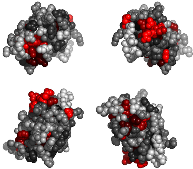
Fig. 2. Residues in 1wzA, colored by their relative importance. Clockwise: front, back, top and bottom views.
