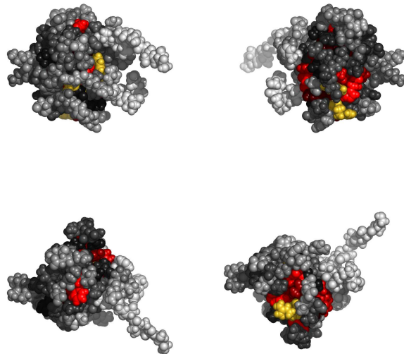
Fig. 2. Residues in 1wquA, colored by their relative importance. Clockwise: front, back, top and bottom views.
