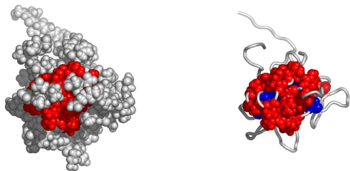
Fig. 4. A possible active surface on the chain 1wquA. The larger cluster it belongs to is shown in blue.
