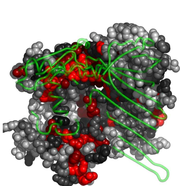
Fig. 5. Residues in 1wruA, at the interface with 1wruA2, colored by their relative importance. 1wruA2 is shown in backbone representation (See Appendix for the coloring scheme for the protein chain 1wruA.)
