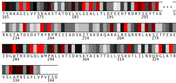
Fig. 2. Residues 165-346 in IwruA colored by their relative importance. (See Appendix, Fig.9, for the coloring scheme.)
