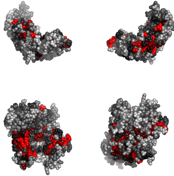
Fig. 3. Residues in IwruA, colored by their relative importance. Clockwise: front, back, top and bottom views.
