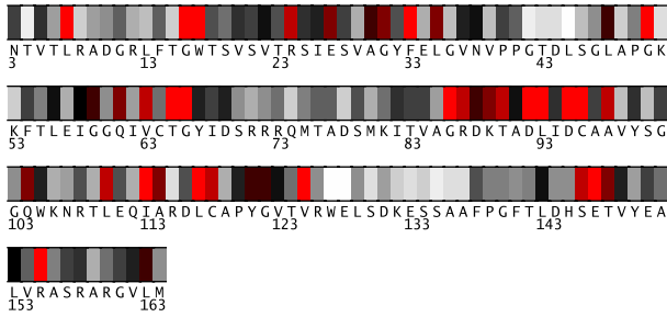
Fig. 1. Residues 3-164 in IwruA colored by their relative importance. (See Appendix, Fig.9, for the coloring scheme.)
