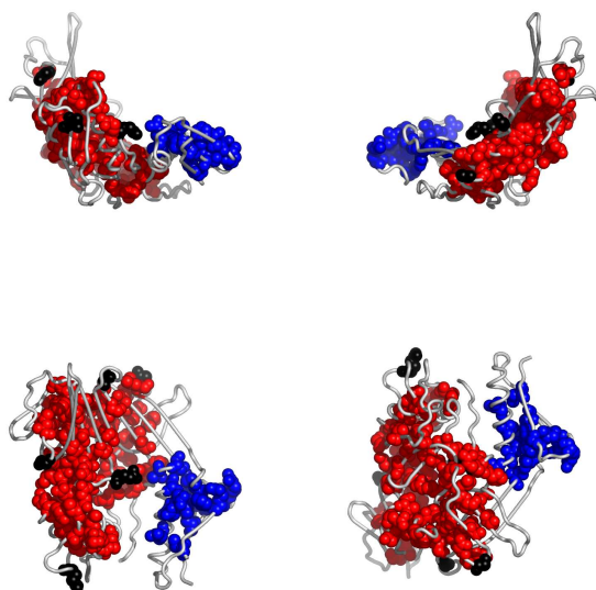
Fig. 4. Residues in 1wruA, colored according to the cluster they belong to: red, followed by blue and yellow are the largest clusters (see Appendix for the coloring scheme). Clockwise: front, back, top and bottom views. The corresponding Pymol script is attached.
