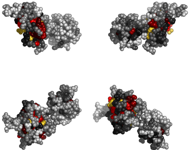
Fig. 1. Residues 63-226 in 1x27B colored by their relative importance. (See Appendix, Fig.9, for the coloring scheme.)
