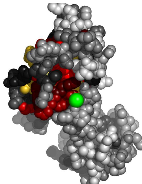
Fig. 6. Residues in 1x27B, at the interface with sodium ion, colored by their relative importance. The ligand (sodium ion) is colored green. Atoms further than 30Å away from the geometric center of the ligand, as well as on the line of sight to the ligand were removed. (See Appendix for the coloring scheme for the protein chain 1x27B.)
