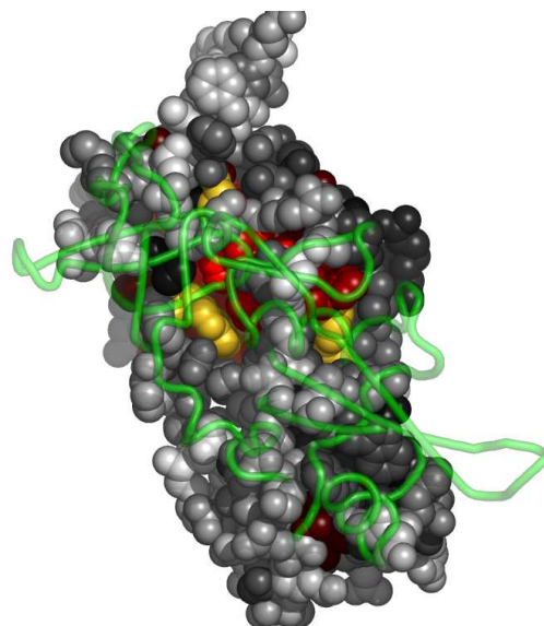
Fig. 5. Residues in 1x27B, at the interface with 1x27D, colored by their relative importance. 1x27D is shown in backbone representation (See Appendix for the coloring scheme for the protein chain 1x27B.)
