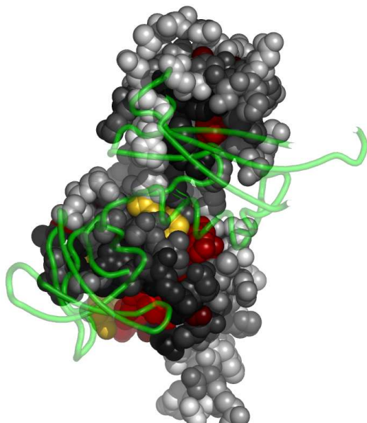
Fig. 7. Residues in 1x27B, at the interface with 1x27C, colored by their relative importance. 1x27C is shown in backbone representation (See Appendix for the coloring scheme for the protein chain 1x27B.)
