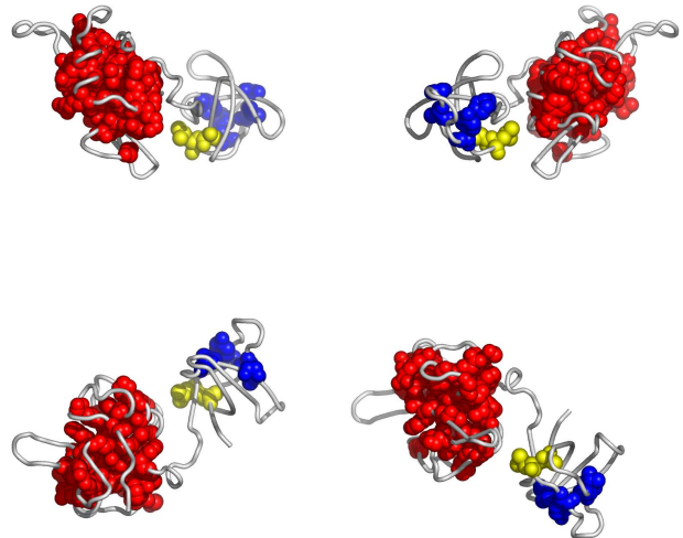
Fig. 3. Residues in 1x27B, colored according to the cluster they belong to: red, followed by blue and yellow are the largest clusters (see Appendix for the coloring scheme). Clockwise: front, back, top and bottom views. The corresponding Pymol script is attached.
