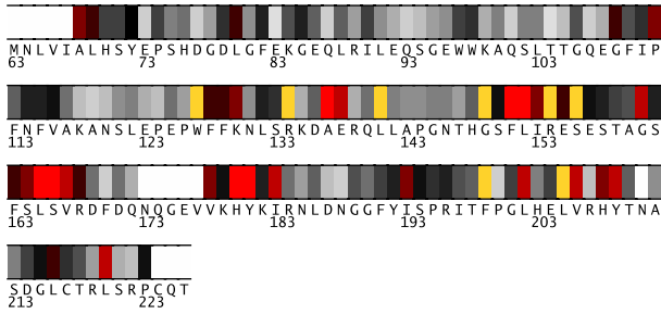
Fig. 1. Residues 63-226 in 1x27B colored by their relative importance. (See Appendix, Fig.9, for the coloring scheme.)
