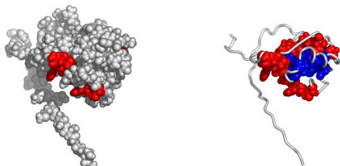
Fig. 4. A possible active surface on the chain 1x4bA. The larger cluster it belongs to is shown in blue.
