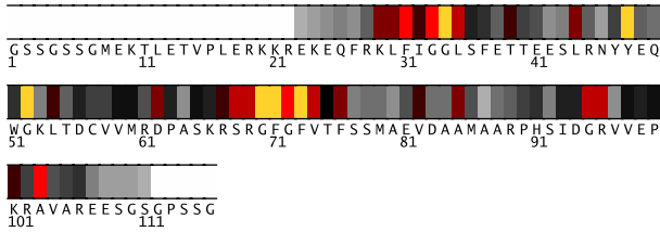
Fig. 1. Residues 1-116 in 1x4bA colored by their relative importance. (See Appendix, Fig.5, for the coloring scheme.)
