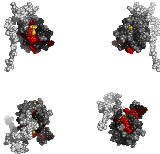
Fig. 2. Residues in 1x4bA, colored by their relative importance. Clockwise: front, back, top and bottom views.
