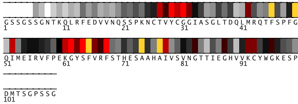
Fig. 1. Residues 1-109 in 1x4gA colored by their relative importance. (See Appendix, Fig.5, for the coloring scheme.)
