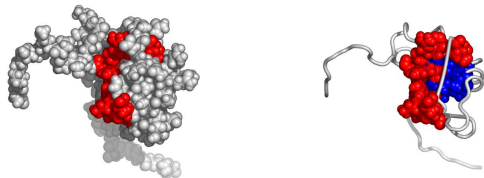
Fig. 4. A possible active surface on the chain 1x4gA. The larger cluster it belongs to is shown in blue.
