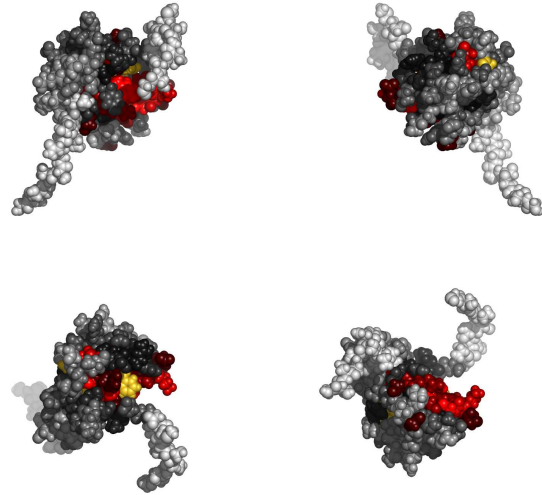
Fig. 2. Residues in 1x4gA, colored by their relative importance. Clockwise: front, back, top and bottom views.
