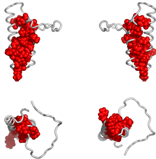
Fig. 3. Residues in 1x59A, colored according to the cluster they belong to: red, followed by blue and yellow are the largest clusters (see Appendix for the coloring scheme). Clockwise: front, back, top and bottom views. The corresponding Pymol script is attached.
