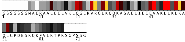
Fig. 1. Residues 1-73 in 1x59A colored by their relative importance. (See Appendix, Fig.5, for the coloring scheme.)
