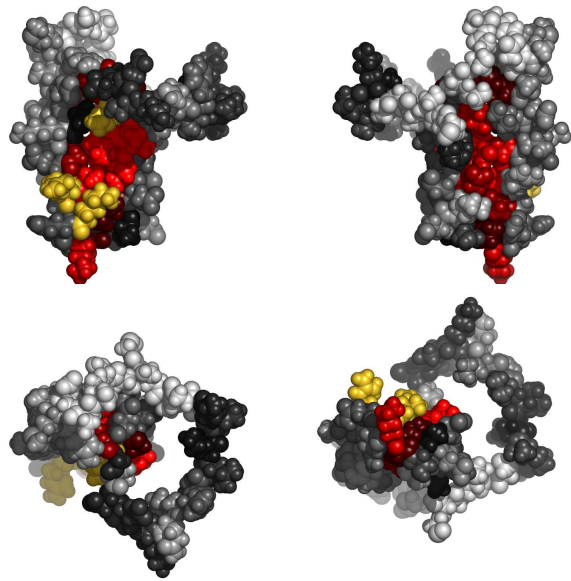
Fig. 2. Residues in 1x59A, colored by their relative importance. Clockwise: front, back, top and bottom views.
