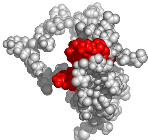
Fig. 4. A possible active surface on the chain 1x59A.
