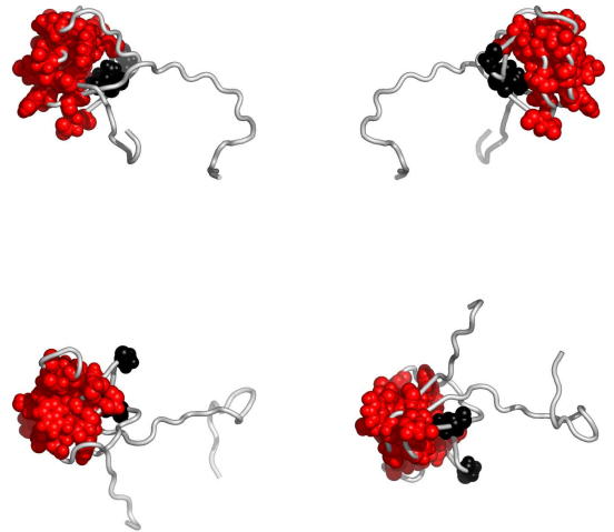
Fig. 3. Residues in 1x69A, colored according to the cluster they belong to: red, followed by blue and yellow are the largest clusters (see Appendix for the coloring scheme). Clockwise: front, back, top and bottom views. The corresponding Pymol script is attached.
