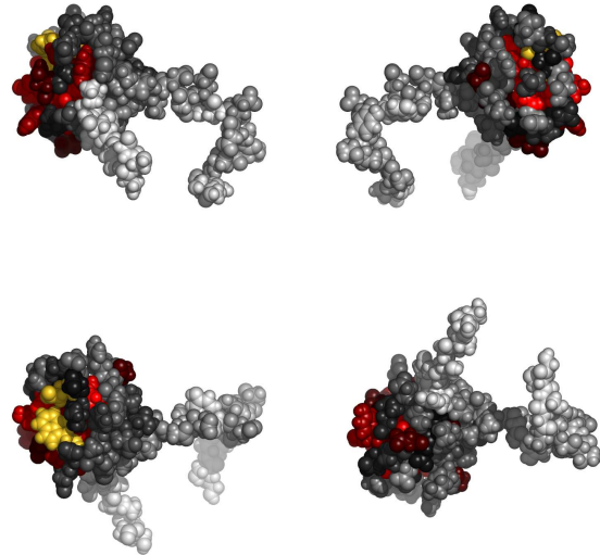
Fig. 2. Residues in 1x69A, colored by their relative importance. Clockwise: front, back, top and bottom views.
