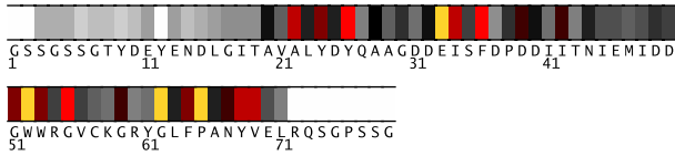
Fig. 1. Residues 1-79 in 1x69A colored by their relative importance. (See Appendix, Fig.5, for the coloring scheme.)
