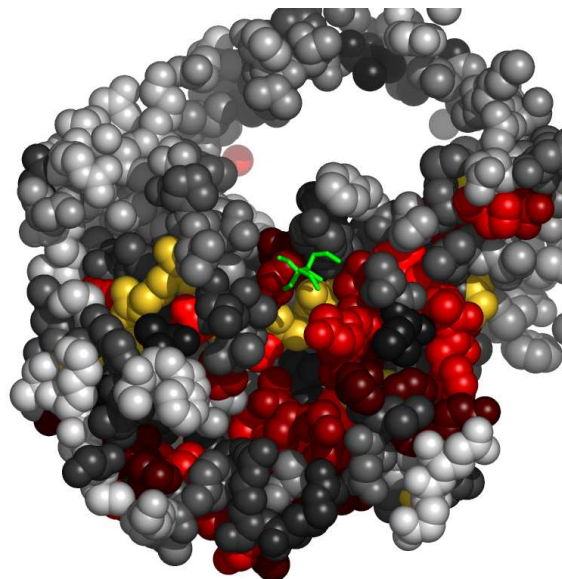
Fig. 6. Residues in 1xa3A, at the interface with BTB, colored by their relative importance. The ligand (BTB) is colored green. Atoms further than 30 Å away from the geometric center of the ligand, as well as on the line of sight to the ligand were removed. (See Appendix for the coloring scheme for the protein chain 1xa3A.)
