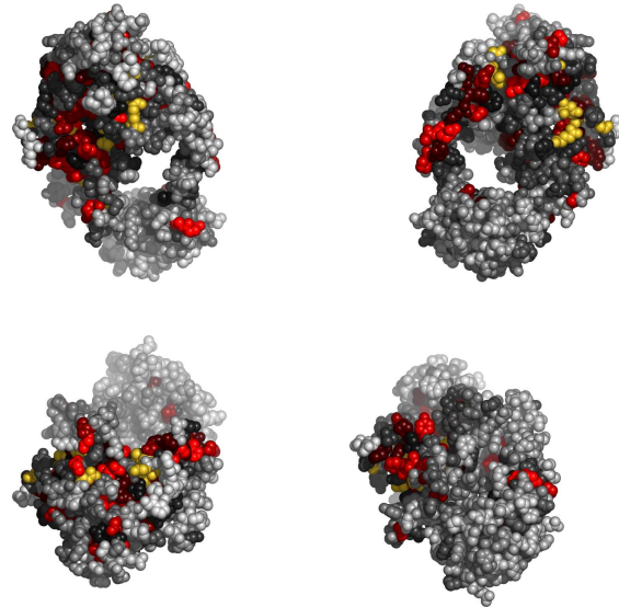
Fig. 3. Residues in 1xa3A, colored by their relative importance. Clockwise: front, back, top and bottom views.
