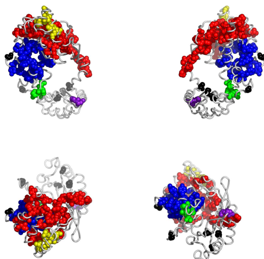
Fig. 4. Residues in 1xa3A, colored according to the cluster they belong to: red, followed by blue and yellow are the largest clusters (see Appendix for the coloring scheme). Clockwise: front, back, top and bottom views. The corresponding Pymol script is attached.
