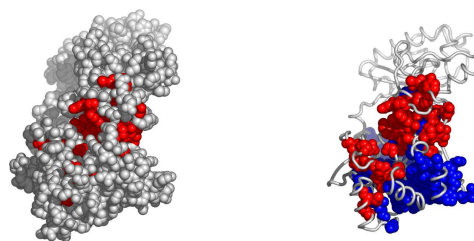
Fig. 9. A possible active surface on the chain 1xa3A. The larger cluster it belongs to is shown in blue.
