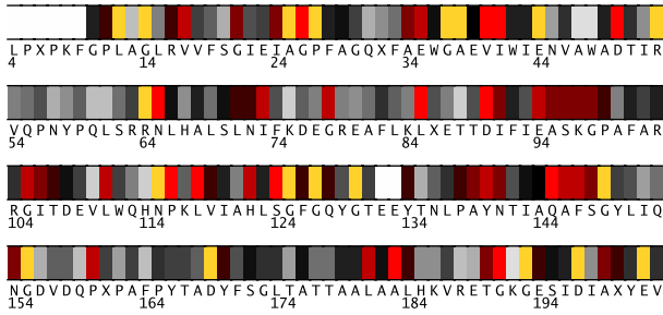
Fig. 1. Residues 4-203 in 1xa3A colored by their relative importance. (See Appendix, Fig.11, for the coloring scheme.)
