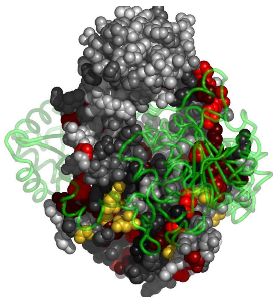
Fig. 8. Residues in 1xa3A, at the interface with 1xa3B, colored by their relative importance. 1xa3B is shown in backbone representation (See Appendix for the coloring scheme for the protein chain 1xa3A.)
