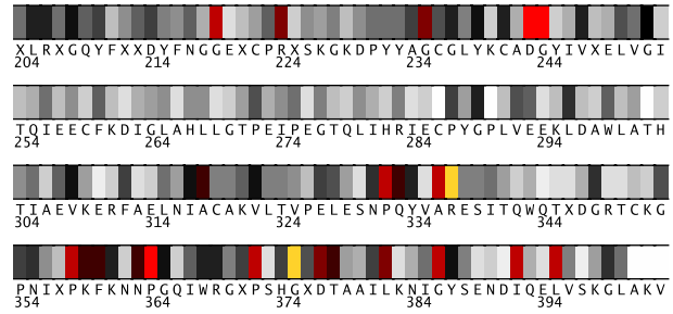
Fig. 2. Residues 204-403 in 1xa3A colored by their relative importance. (See Appendix, Fig.11, for the coloring scheme.)
