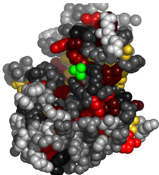
Fig. 7. Residues in 1xa3A, at the interface with sulfate ion, colored by their relative importance. The ligand (sulfate ion) is colored green. Atoms further than 30Å away from the geometric center of the ligand, as well as on the line of sight to the ligand were removed. (See Appendix for the coloring scheme for the protein chain 1xa3A.)
