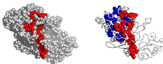
Fig. 10. Another possible active surface on the chain 1xa3A. The larger cluster it belongs to is shown in blue.
