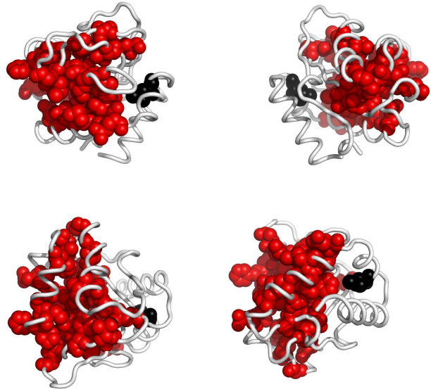
Fig. 3. Residues in 1xizB, colored according to the cluster they belong to: red, followed by blue and yellow are the largest clusters (see Appendix for the coloring scheme). Clockwise: front, back, top and bottom views. The corresponding Pymol script is attached.
