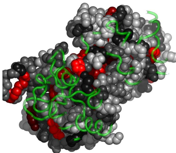
Fig. 5. Residues in 1yh3A, at the interface with 1yh3B, colored by their relative importance. 1yh3B is shown in backbone representation (See Appendix for the coloring scheme for the protein chain 1yh3A.)
