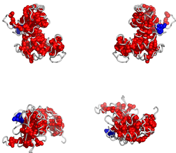
Fig. 4. Residues in 1yh3A, colored according to the cluster they belong to: red, followed by blue and yellow are the largest clusters (see Appendix for the coloring scheme). Clockwise: front, back, top and bottom views. The corresponding Pymol script is attached.
