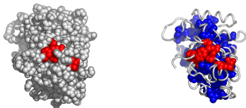
Fig. 6. A possible active surface on the chain 1yh3A. The larger cluster it belongs to is shown in blue.
