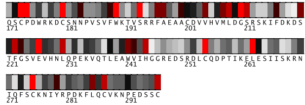
Fig. 2. Residues 171-296 in 1yh3A colored by their relative importance. (See Appendix, Fig.8, for the coloring scheme.)
