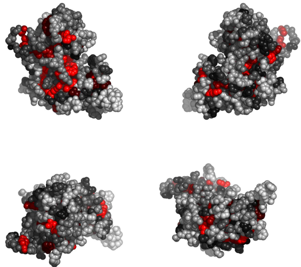
Fig. 3. Residues in 1yh3A, colored by their relative importance. Clockwise: front, back, top and bottom views.
