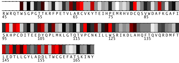
Fig. 1. Residues 45-170 in 1yh3A colored by their relative importance. (See Appendix, Fig.8, for the coloring scheme.)
