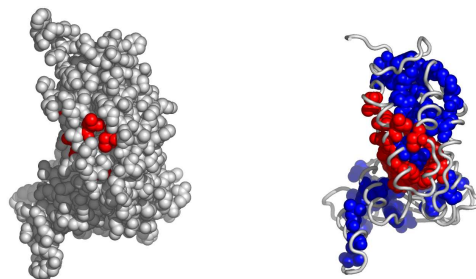
Fig. 7. Another possible active surface on the chain 1yh3A. The larger cluster it belongs to is shown in blue.
