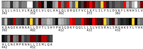
Fig. 2. Residues 342-459 in 1ymtA colored by their relative importance. (See Appendix, Fig.8, for the coloring scheme.)
