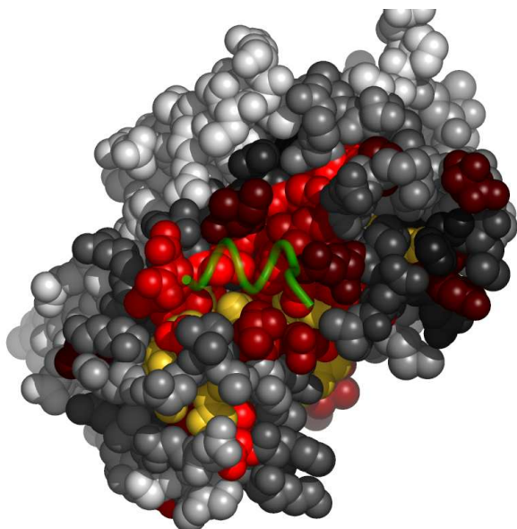
Fig. 5. Residues in 1ymtA, at the interface with 1ymtB, colored by their relative importance. 1ymtB is shown in backbone representation (See Appendix for the coloring scheme for the protein chain 1ymtA.)
