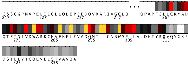
Fig. 1. Residues 217-341 in 1ymtA colored by their relative importance. (See Appendix, Fig.8, for the coloring scheme.)
