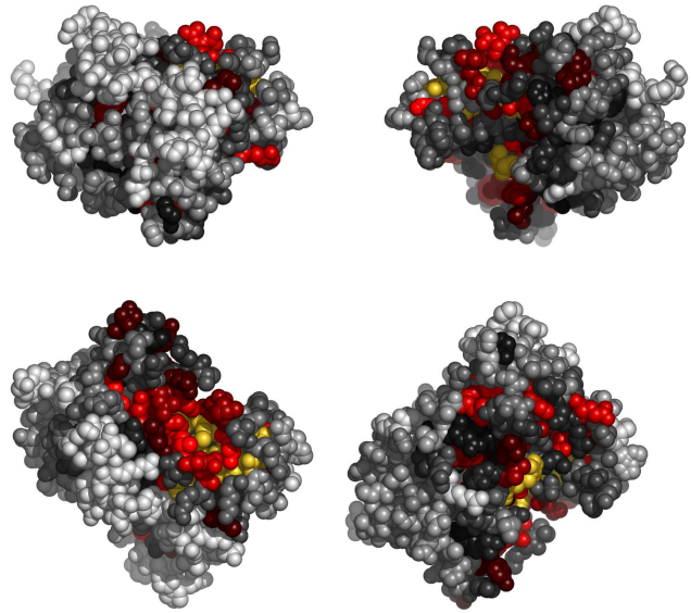
Fig. 3. Residues in 1ymtA, colored by their relative importance. Clockwise: front, back, top and bottom views.
