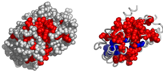
Fig. 6. Residues in 1ymtA, at the interface with DR9, colored by their relative importance. The ligand (DR9) is colored green. Atoms further than 30Å away from the geometric center of the ligand, as well as on the line of sight to the ligand were removed. (See Appendix for the coloring scheme for the protein chain 1ymtA.)
