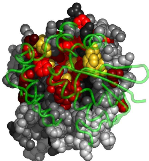
Fig. 5. Residues in 1yzxA, at the interface with 1yzxB, colored by their relative importance. 1yzxB is shown in backbone representation (See Appendix for the coloring scheme for the protein chain 1yzxA.)
