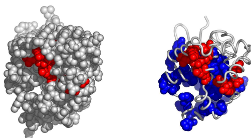
Fig. 8. A possible active surface on the chain 1yzaA. The larger cluster it belongs to is shown in blue.
