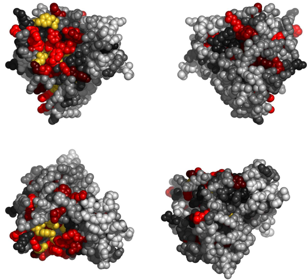
Fig. 3. Residues in 1yzaA, colored by their relative importance. Clockwise: front, back, top and bottom views.
