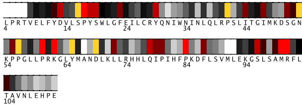
Fig. 1. Residues 4-112 in 1yzaA colored by their relative importance. (See Appendix, Fig.9, for the coloring scheme.)
