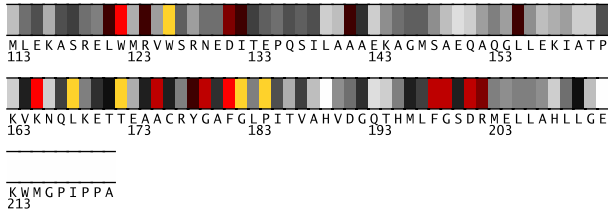
Fig. 2. Residues 113-221 in 1yzaA colored by their relative importance. (See Appendix, Fig.9, for the coloring scheme.)
