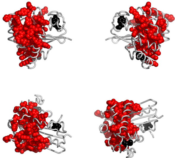
Fig. 4. Residues in 1yzaA, colored according to the cluster they belong to: red, followed by blue and yellow are the largest clusters (see Appendix for the coloring scheme). Clockwise: front, back, top and bottom views. The corresponding Pymol script is attached.
