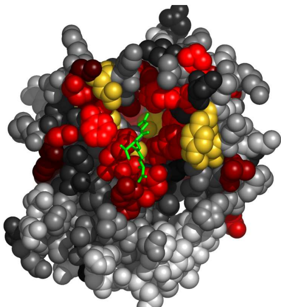
Fig. 7. Residues in 1yzaA, at the interface with GSF, colored by their relative importance. The ligand (GSF) is colored green. Atoms further than 30\text{\AA} away from the geometric center of the ligand, as well as on the line of sight to the ligand were removed. (See Appendix for the coloring scheme for the protein chain 1yzaA.)
