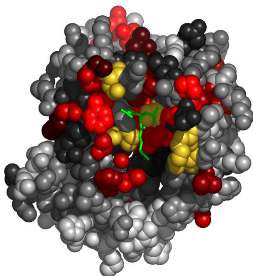
Fig. 6. Residues in 1yzxA, at the interface with GSF, colored by their relative importance. The ligand (GSF) is colored green. Atoms further than 30Å away from the geometric center of the ligand, as well as on the line of sight to the ligand were removed. (See Appendix for the coloring scheme for the protein chain 1yzxA.)
