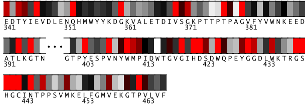
Fig. 2. Residues 341-466 in IzatA colored by their relative importance. (See Appendix, Fig.7, for the coloring scheme.)
