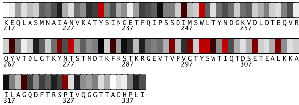
Fig. 1. Residues 217-340 in IzatA colored by their relative importance. (See Appendix, Fig.7, for the coloring scheme.)
