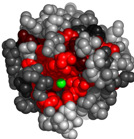
Fig. 5. Residues in 1zatA, at the interface with zinc ion, colored by their relative importance. The ligand (zinc ion) is colored green. Atoms further than 30Å away from the geometric center of the ligand, as well as on the line of sight to the ligand were removed. (See Appendix for the coloring scheme for the protein chain 1zatA.)
