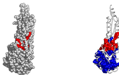
Fig. 6. A possible active surface on the chain 1zatA. The larger cluster it belongs to is shown in blue.
