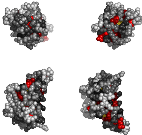
Fig. 2. Residues in 1zoxA, colored by their relative importance. Clockwise: front, back, top and bottom views.
