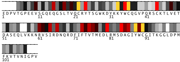
Fig. 1. Residues 1-110 in 1zoxA colored by their relative importance. (See Appendix, Fig.5, for the coloring scheme.)
