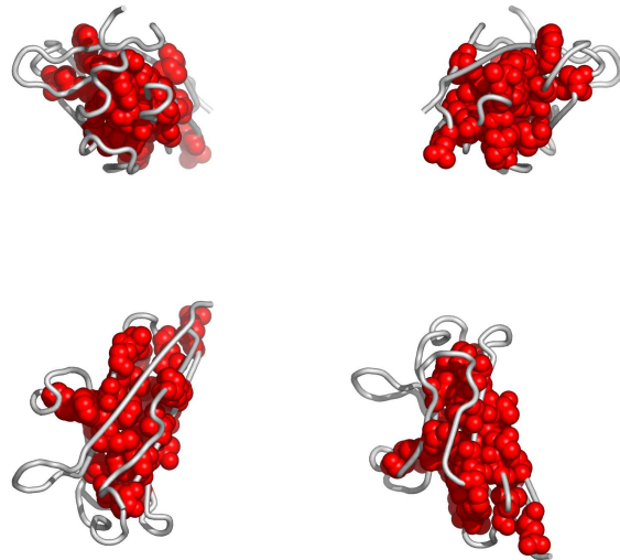
Fig. 3. Residues in 1zoxA, colored according to the cluster they belong to: red, followed by blue and yellow are the largest clusters (see Appendix for the coloring scheme). Clockwise: front, back, top and bottom views. The corresponding Pymol script is attached.
