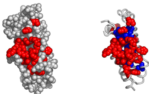
Fig. 4. A possible active surface on the chain 1zv4X. The larger cluster it belongs to is shown in blue.
