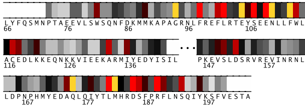
Fig. 1. Residues 66-204 in 1zv4X colored by their relative importance. (See Appendix, Fig.5, for the coloring scheme.)
