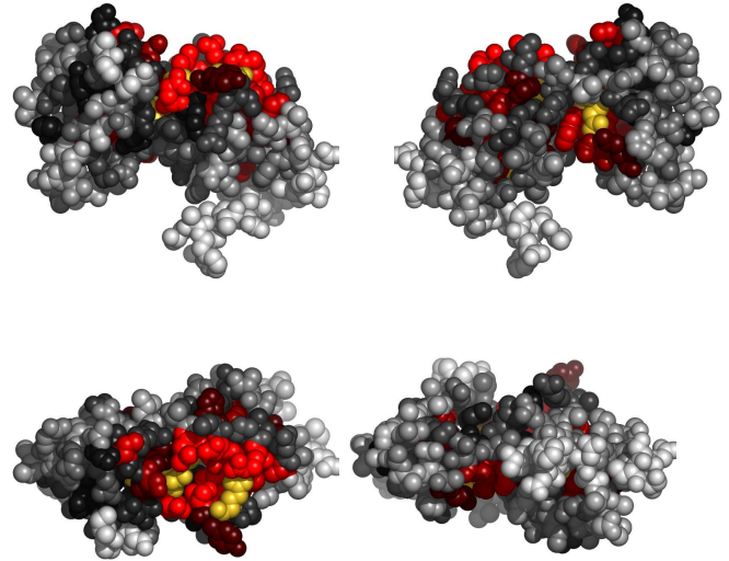
Fig. 1. Residues 66-204 in 1zv4X colored by their relative importance. (See Appendix, Fig.5, for the coloring scheme.)
