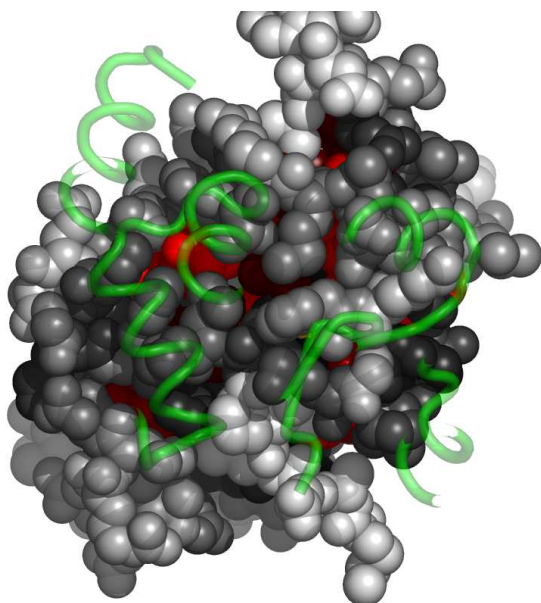
Fig. 6. Residues in 1zzwA, at the interface with 1zzwB, colored by their relative importance. 1zzwB is shown in backbone representation (See Appendix for the coloring scheme for the protein chain 1zzwA.)
