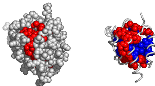
Fig. 7. A possible active surface on the chain 1zzwA. The larger cluster it belongs to is shown in blue.
