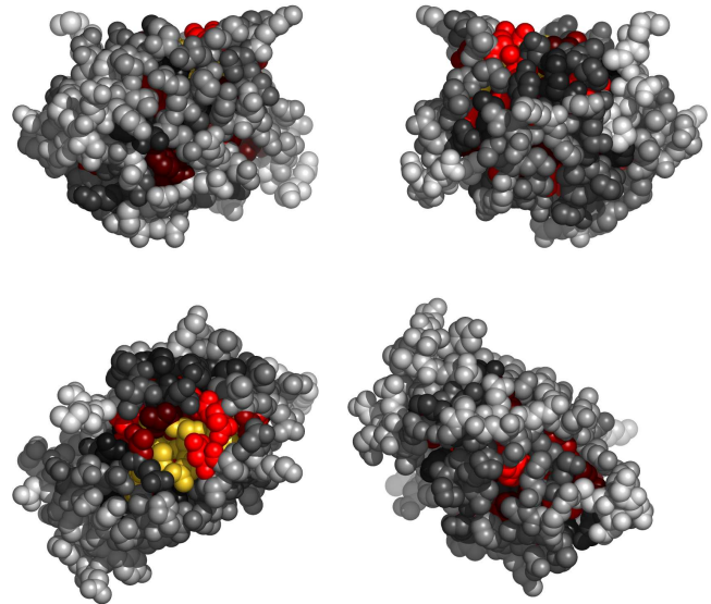
Fig. 2. Residues in IzzwA, colored by their relative importance. Clockwise: front, back, top and bottom views.
