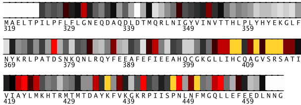
Fig. 1. Residues 319-465 in IzzwA colored by their relative importance. (See Appendix, Fig.8, for the coloring scheme.)
