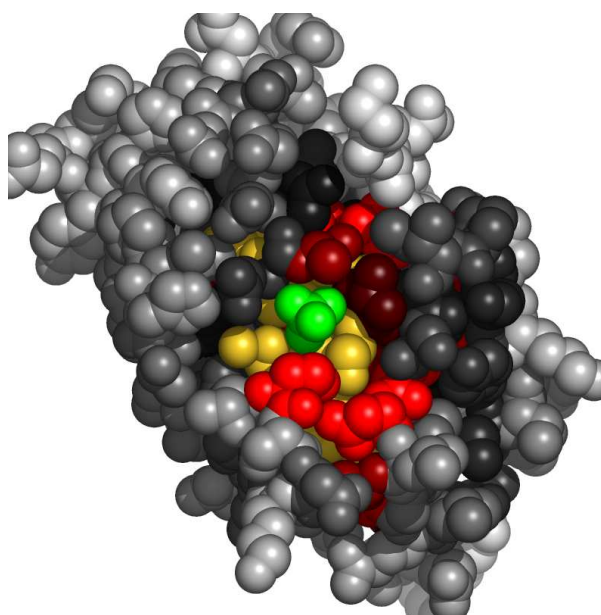
Fig. 5. Residues in 1zzwA, at the interface with sulfate ion, colored by their relative importance. The ligand (sulfate ion) is colored green. Atoms further than 30Å away from the geometric center of the ligand, as well as on the line of sight to the ligand were removed. (See Appendix for the coloring scheme for the protein chain 1zzwA.)
