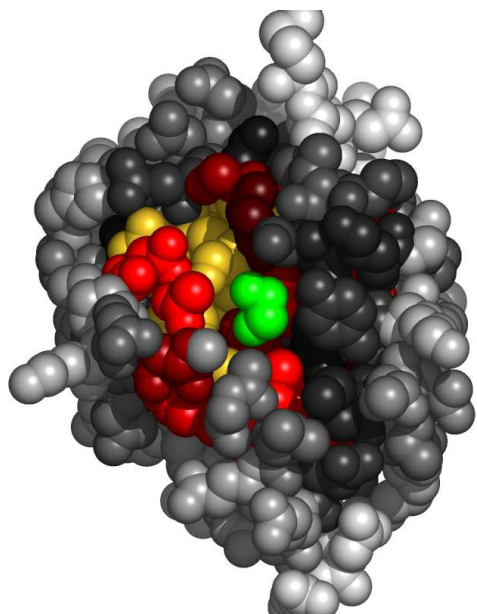
Fig. 4. Residues in 1zzwA, at the interface with 1,2-ethanediol, colored by their relative importance. The ligand (1,2-ethanediol) is colored green. Atoms further than 30Å away from the geometric center of the ligand, as well as on the line of sight to the ligand were removed. (See Appendix for the coloring scheme for the protein chain 1zzwA.)
