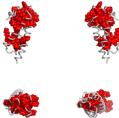
Fig. 2. Residues in 2a7oA, colored by their relative importance. Clockwise: front, back, top and bottom views.
