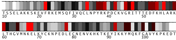
Fig. 1. Residues 10-109 in 2a7oA colored by their relative importance. (See Appendix, Fig.5, for the coloring scheme.)
