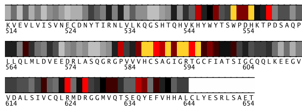
Fig. 2. Residues 514-655 in 2a8bA colored by their relative importance. (See Appendix, Fig.6, for the coloring scheme.)
