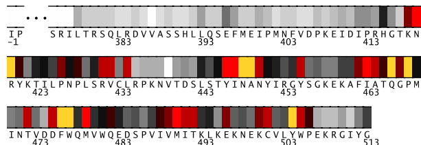
Fig. 1. Residues -1-513 in 2a8bA colored by their relative importance. (See Appendix, Fig.6, for the coloring scheme.)
