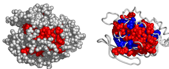
Fig. 5. A possible active surface on the chain 2a8bA. The larger cluster it belongs to is shown in blue.
