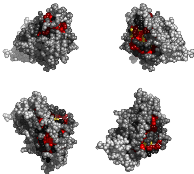
Fig. 3. Residues in 2a8bA, colored by their relative importance. Clockwise: front, back, top and bottom views.
