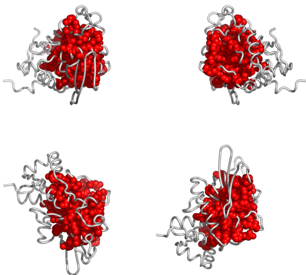
Fig. 4. Residues in 2a8bA, colored according to the cluster they belong to: red, followed by blue and yellow are the largest clusters (see Appendix for the coloring scheme). Clockwise: front, back, top and bottom views. The corresponding Pymol script is attached.
