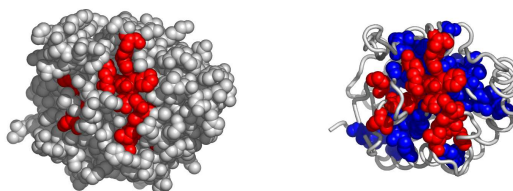
Fig. 6. A possible active surface on the chain 2apjA. The larger cluster it belongs to is shown in blue.
