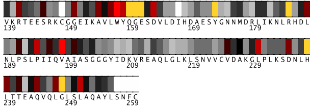
Fig. 2. Residues 139-260 in 2apjA colored by their relative importance. (See Appendix, Fig.7, for the coloring scheme.)
