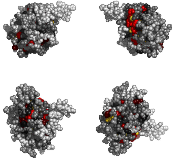
Fig. 3. Residues in 2apjA, colored by their relative importance. Clockwise: front, back, top and bottom views.
