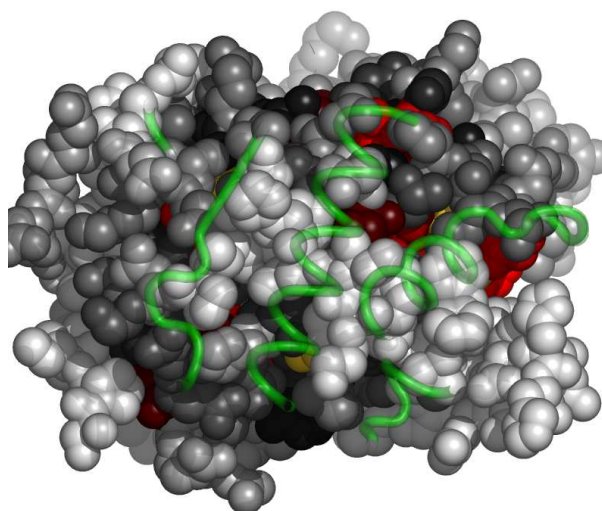
Fig. 5. Residues in 2apjA, at the interface with 2apjB, colored by their relative importance. 2apjB is shown in backbone representation (See Appendix for the coloring scheme for the protein chain 2apjA.)
