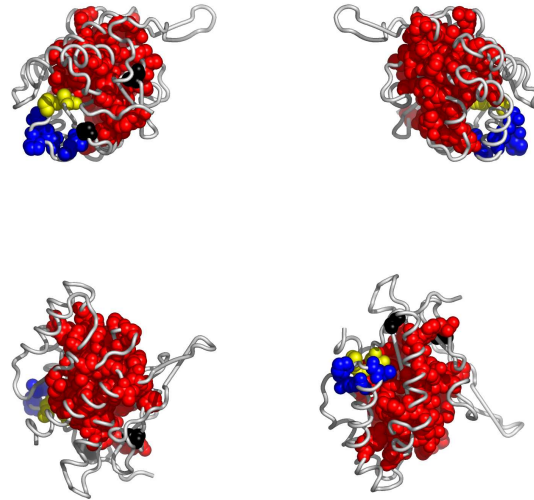
Fig. 4. Residues in 2apjA, colored according to the cluster they belong to: red, followed by blue and yellow are the largest clusters (see Appendix for the coloring scheme). Clockwise: front, back, top and bottom views. The corresponding Pymol script is attached.
