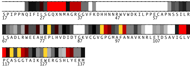
Fig. 1. Residues 17-138 in 2apjA colored by their relative importance. (See Appendix, Fig.7, for the coloring scheme.)
