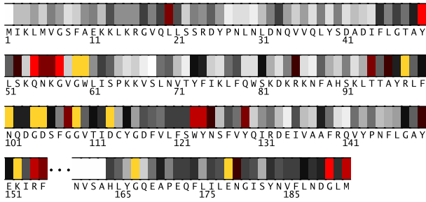
Fig. 1. Residues 1-192 in 2b78A colored by their relative importance. (See Appendix, Fig.6, for the coloring scheme.)
