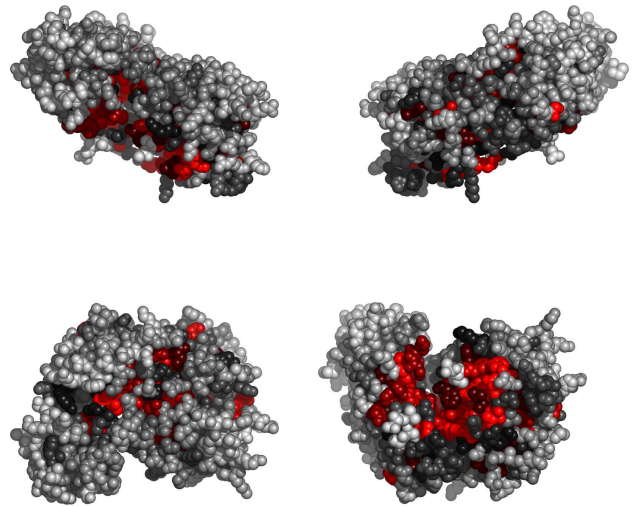
Fig. 1. Residues 1-192 in 2b78A colored by their relative importance. (See Appendix, Fig.6, for the coloring scheme.)
