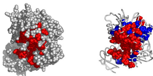
Fig. 5. A possible active surface on the chain 2b78A. The larger cluster it belongs to is shown in blue.
