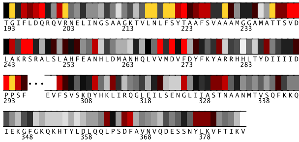
Fig. 2. Residues 193-385 in 2b78A colored by their relative importance. (See Appendix, Fig.6, for the coloring scheme.)
