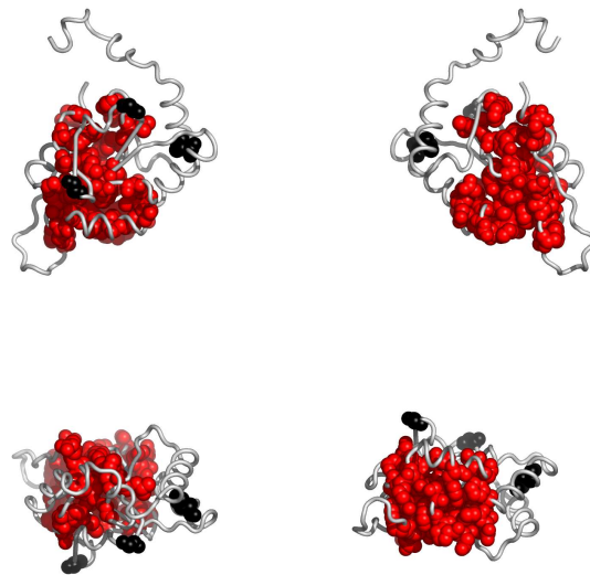
Fig. 2. Residues in 2b7jD, colored by their relative importance. Clockwise: front, back, top and bottom views.
