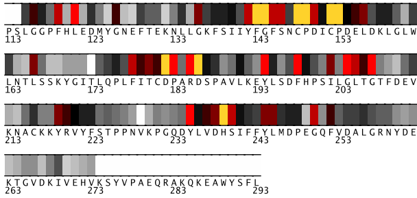
Fig. 1. Residues 113-293 in 2b7jD colored by their relative importance. (See Appendix, Fig.9, for the coloring scheme.)
