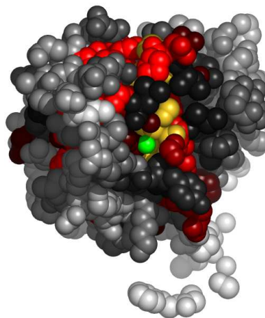
Fig. 4. Residues in 2b7jD, at the interface with copper (ii) ion, colored by their relative importance. The ligand (copper (ii) ion) is colored green. Atoms further than 30 Å away from the geometric center of the ligand, as well as on the line of sight to the ligand were removed. (See Appendix for the coloring scheme for the protein chain 2b7jD.)
