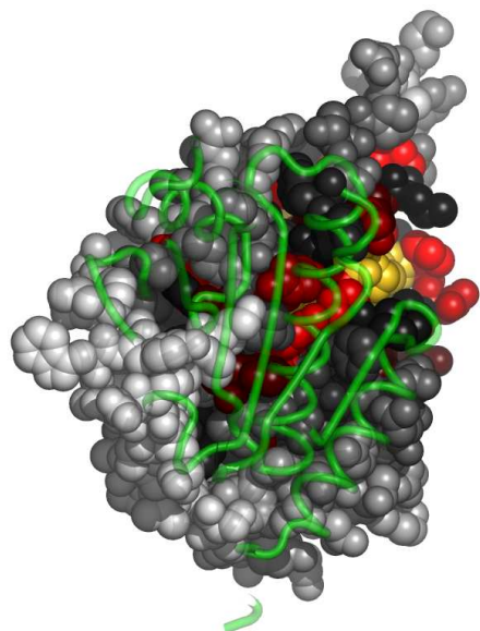
Fig. 6. Residues in 2b7jD, at the interface with 2b7jC, colored by their relative importance. 2b7jC is shown in backbone representation (See Appendix for the coloring scheme for the protein chain 2b7jD.)
