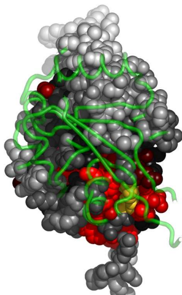
Fig. 5. Residues in 2b7jD, at the interface with 2b7jB, colored by their relative importance. 2b7jB is shown in backbone representation (See Appendix for the coloring scheme for the protein chain 2b7jD.)
