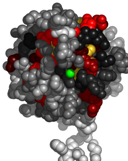
Fig. 7. Residues in 2b7jD, at the interface with copper (ii) ion, colored by their relative importance. The ligand (copper (ii) ion) is colored green. Atoms further than 30 Å away from the geometric center of the ligand, as well as on the line of sight to the ligand were removed. (See Appendix for the coloring scheme for the protein chain 2b7jD.)
