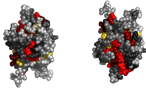
Fig. 2. Residues in 2bmjA, colored by their relative importance. Clockwise: front, back, top and bottom views.
