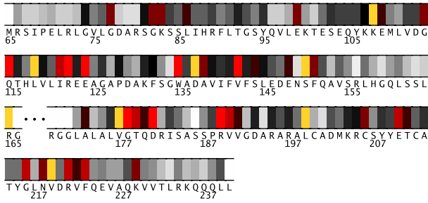
Fig. 1. Residues 65-240 in 2bmjA colored by their relative importance. (See Appendix, Fig.5, for the coloring scheme.)
