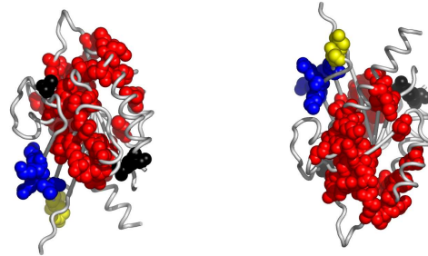
Fig. 3. Residues in 2bmjA, colored according to the cluster they belong to: red, followed by blue and yellow are the largest clusters (see Appendix for the coloring scheme). Clockwise: front, back, top and bottom views. The corresponding Pymol script is attached.
