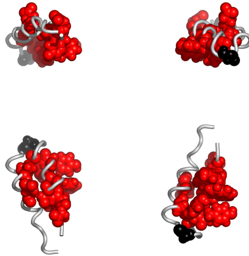
Fig. 3. Residues in 2bn5A, colored according to the cluster they belong to: red, followed by blue and yellow are the largest clusters (see Appendix for the coloring scheme). Clockwise: front, back, top and bottom views. The corresponding Pymol script is attached.
