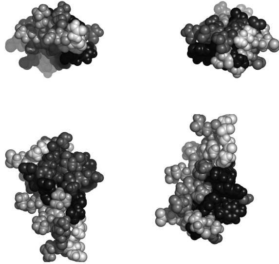
Fig. 2. Residues in 2bn5A, colored by their relative importance. Clockwise: front, back, top and bottom views.
