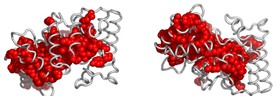
Fig. 4. Residues in 2bp1A, colored according to the cluster they belong to: red, followed by blue and yellow are the largest clusters (see Appendix for the coloring scheme). Clockwise: front, back, top and bottom views. The corresponding Pymol script is attached.
