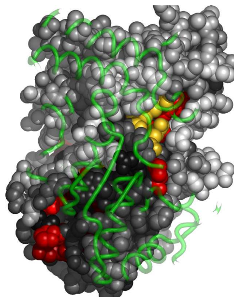
Fig. 5. Residues in 2bp1A, at the interface with 2bp1B, colored by their relative importance. 2bp1B is shown in backbone representation (See Appendix for the coloring scheme for the protein chain 2bp1A.)
