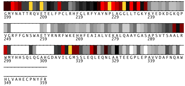
Fig. 2. Residues 199-360 in 2bp1A colored by their relative importance. (See Appendix, Fig.9, for the coloring scheme.)
