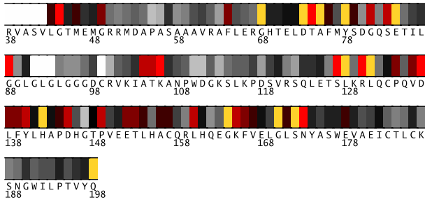
Fig. 1. Residues 38-198 in 2bp1A colored by their relative importance. (See Appendix, Fig.9, for the coloring scheme.)
