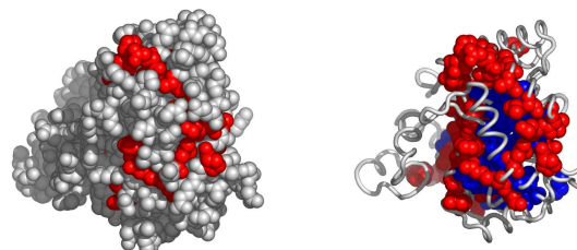
Fig. 8. A possible active surface on the chain 2bp1A. The larger cluster it belongs to is shown in blue.
