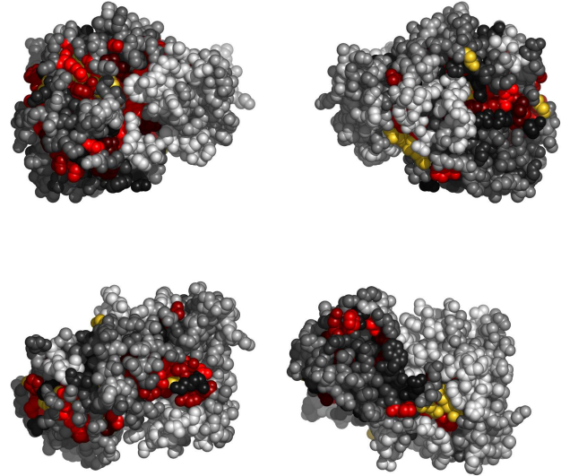
Fig. 3. Residues in 2bp1A, colored by their relative importance. Clockwise: front, back, top and bottom views.
