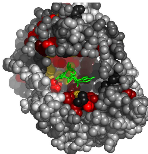
Fig. 6. Residues in 2bp1A, at the interface with NDP, colored by their relative importance. The ligand (NDP) is colored green. Atoms further than 30Å away from the geometric center of the ligand, as well as on the line of sight to the ligand were removed. (See Appendix for the coloring scheme for the protein chain 2bp1A.)
