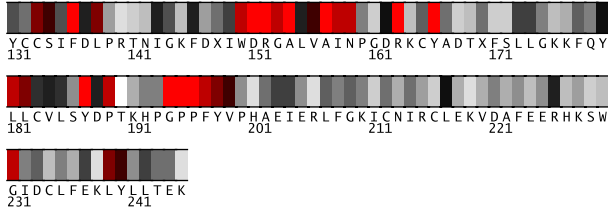
Fig. 2. Residues 131-245 in 2bzdA colored by their relative importance. (See Appendix, Fig.7, for the coloring scheme.)
