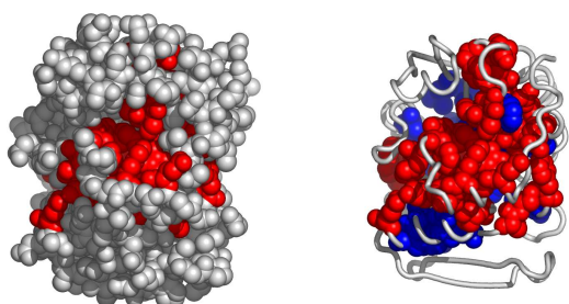
Fig. 6. A possible active surface on the chain 2bzgA. The larger cluster it belongs to is shown in blue.
