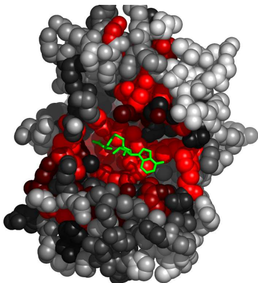
Fig. 5. Residues in 2bzgA, at the interface with SAH, colored by their relative importance. The ligand (SAH) is colored green. Atoms further than 30Å away from the geometric center of the ligand, as well as on the line of sight to the ligand were removed. (See Appendix for the coloring scheme for the protein chain 2bzgA.)
