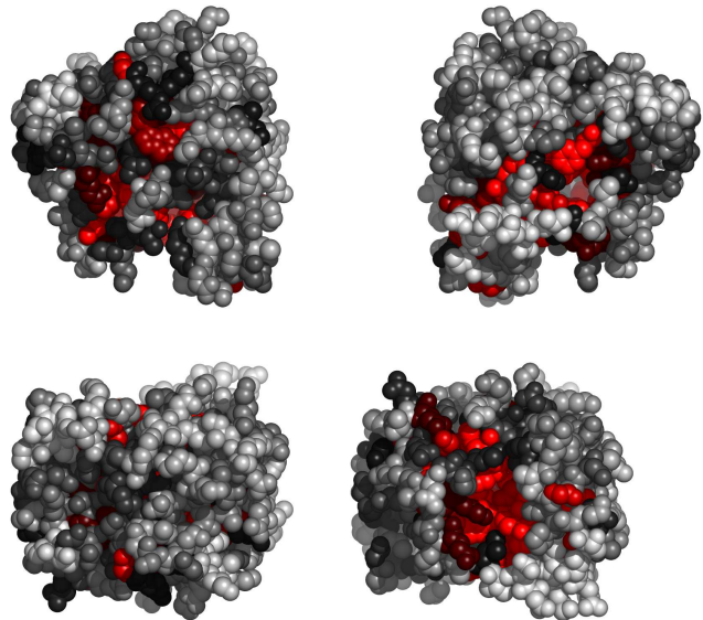
Fig. 3. Residues in 2bzdA, colored by their relative importance. Clockwise: front, back, top and bottom views.
