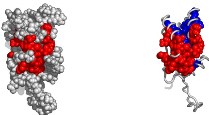
Fig. 4. A possible active surface on the chain 2cq9A. The larger cluster it belongs to is shown in blue.
