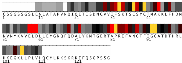
Fig. 1. Residues 1-130 in 2cq9A colored by their relative importance. (See Appendix, Fig.5, for the coloring scheme.)
