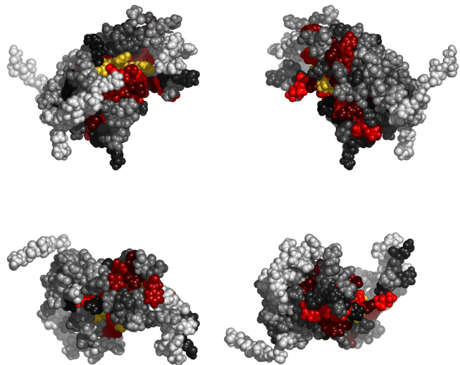
Fig. 1. Residues 1-146 in 2cskA colored by their relative importance. (See Appendix, Fig.5, for the coloring scheme.)
