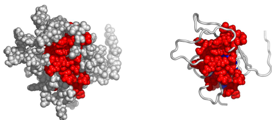
Fig. 4. A possible active surface on the chain 2cskA. The larger cluster it belongs to is shown in blue.
