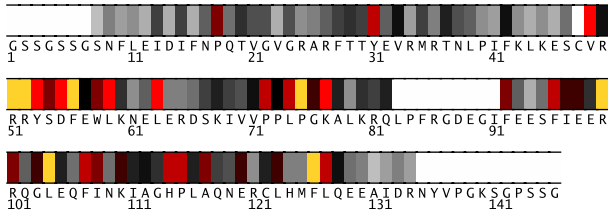
Fig. 1. Residues 1-146 in 2cskA colored by their relative importance. (See Appendix, Fig.5, for the coloring scheme.)
