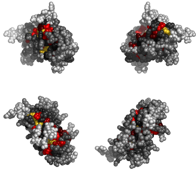
Fig. 1. Residues -4-165 in 2cyxA colored by their relative importance. (See Appendix, Fig.6, for the coloring scheme.)
