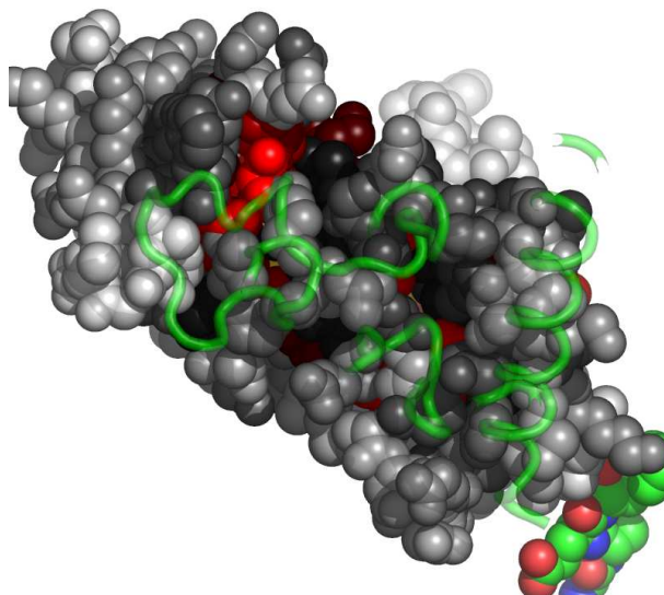
Fig. 4. Residues in 2cyxA, at the interface with 2cyxB, colored by their relative importance. 2cyxB is shown in backbone representation (See Appendix for the coloring scheme for the protein chain 2cyxA.)
