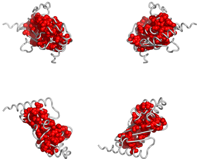
Fig. 3. Residues in 2cyxA, colored according to the cluster they belong to: red, followed by blue and yellow are the largest clusters (see Appendix for the coloring scheme). Clockwise: front, back, top and bottom views. The corresponding Pymol script is attached.
