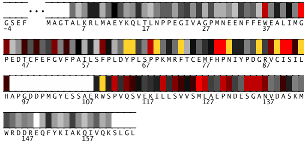
Fig. 1. Residues -4-165 in 2cyxA colored by their relative importance. (See Appendix, Fig.6, for the coloring scheme.)
