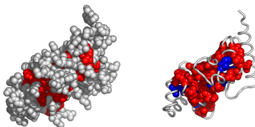
Fig. 4. Residues in 2cyxA, at the interface with 2cyxB, colored by their relative importance. 2cyxB is shown in backbone representation (See Appendix for the coloring scheme for the protein chain 2cyxA.)
