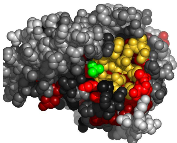
Fig. 6. Residues in 2czhA, at the interface with phosphate ion, colored by their relative importance. The ligand (phosphate ion) is colored green. Atoms further than 30Å away from the geometric center of the ligand, as well as on the line of sight to the ligand were removed. (See Appendix for the coloring scheme for the protein chain 2czhA.)
