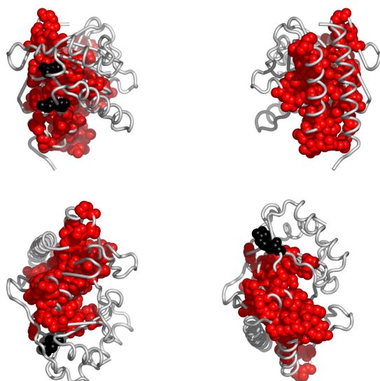
Fig. 4. Residues in 2czhA, colored according to the cluster they belong to: red, followed by blue and yellow are the largest clusters (see Appendix for the coloring scheme). Clockwise: front, back, top and bottom views. The corresponding Pymol script is attached.
