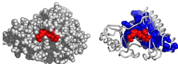
Fig. 8. Another possible active surface on the chain 2czhA. The larger cluster it belongs to is shown in blue.
