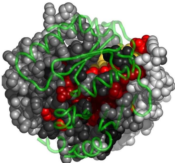
Fig. 5. Residues in 2czhA, at the interface with 2czhB, colored by their relative importance. 2czhB is shown in backbone representation (See Appendix for the coloring scheme for the protein chain 2czhA.)
