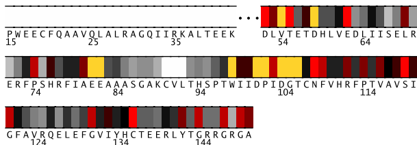
Fig. 1. Residues 15-150 in 2czhA colored by their relative importance. (See Appendix, Fig.9, for the coloring scheme.)
