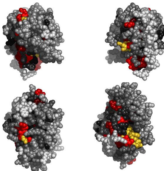
Fig. 3. Residues in 2czhA, colored by their relative importance. Clockwise: front, back, top and bottom views.
