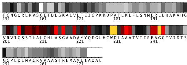
Fig. 2. Residues 151-277 in 2czhA colored by their relative importance. (See Appendix, Fig.9, for the coloring scheme.)
