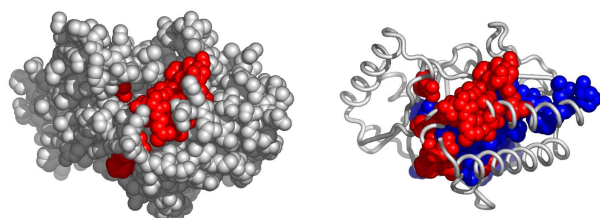
Fig. 7. A possible active surface on the chain 2czhA. The larger cluster it belongs to is shown in blue.
