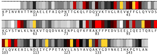
Fig. 1. Residues 3-149 in 2d11A colored by their relative importance. (See Appendix, Fig.7, for the coloring scheme.)
