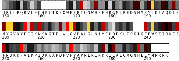
Fig. 2. Residues 150-296 in 2d11A colored by their relative importance. (See Appendix, Fig.7, for the coloring scheme.)
