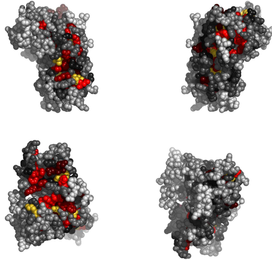
Fig. 3. Residues in 2d11A, colored by their relative importance. Clockwise: front, back, top and bottom views.
