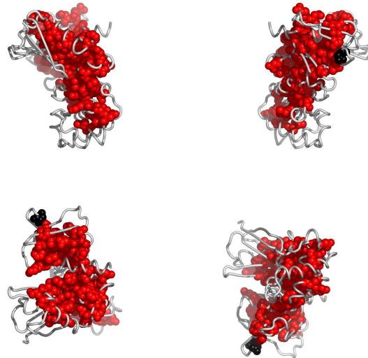
Fig. 4. Residues in 2d11A, colored according to the cluster they belong to: red, followed by blue and yellow are the largest clusters (see Appendix for the coloring scheme). Clockwise: front, back, top and bottom views. The corresponding Pymol script is attached.
