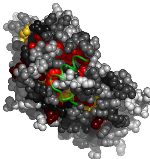
Fig. 5. Residues in 2d11A, at the interface with 2d11F, colored by their relative importance. 2d11F is shown in backbone representation (See Appendix for the coloring scheme for the protein chain 2d11A.)
