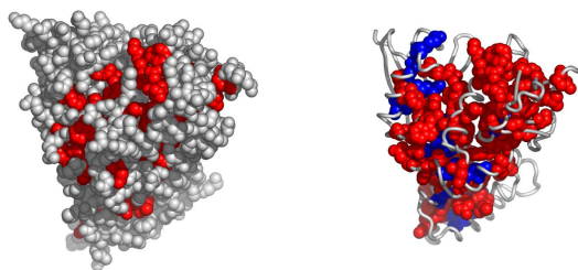
Fig. 6. A possible active surface on the chain 2d11A. The larger cluster it belongs to is shown in blue.
