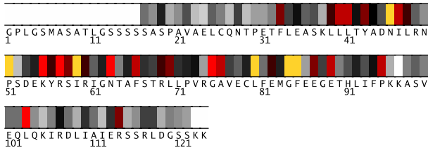
Fig. 1. Residues 1-124 in 2d5uA colored by their relative importance. (See Appendix, Fig.5, for the coloring scheme.)
