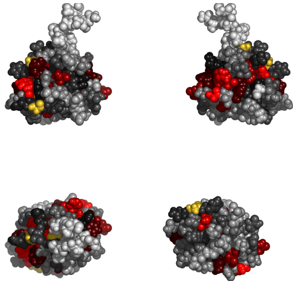
Fig. 1. Residues 1-93 in 2dadA colored by their relative importance. (See Appendix, Fig.5, for the coloring scheme.)
