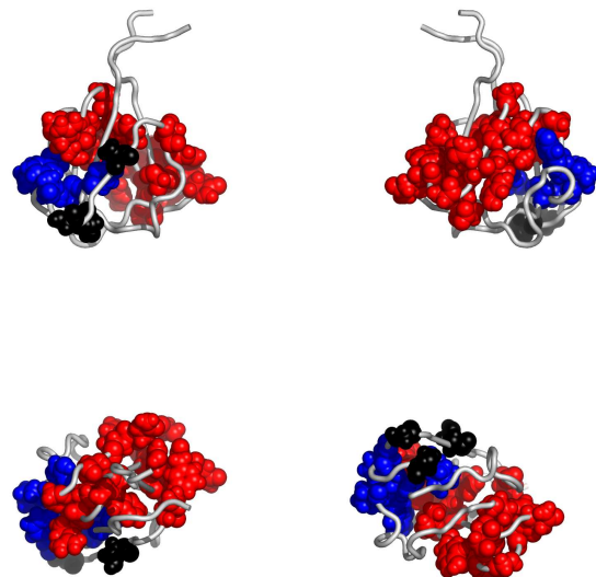
Fig. 2. Residues in 2dadA, colored by their relative importance. Clockwise: front, back, top and bottom views.
