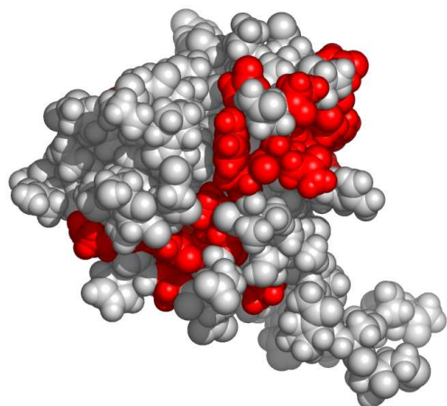
Fig. 4. A possible active surface on the chain 2dadA.
