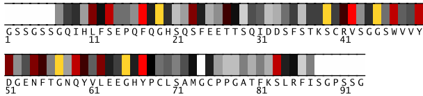
Fig. 1. Residues 1-93 in 2dadA colored by their relative importance. (See Appendix, Fig.5, for the coloring scheme.)
