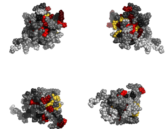
Fig. 1. Residues 1-125 in 2dhjA colored by their relative importance. (See Appendix, Fig.5, for the coloring scheme.)
