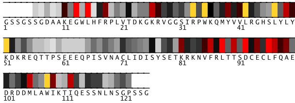
Fig. 1. Residues 1-125 in 2dhjA colored by their relative importance. (See Appendix, Fig.5, for the coloring scheme.)
